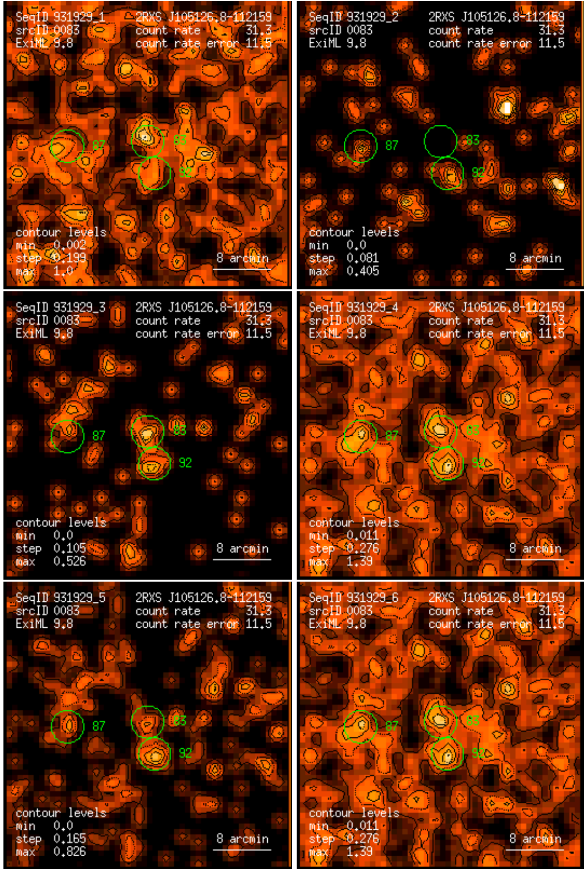
Figure 83: RASS 931929: detection 0083: band rate images, Gaussian filter: (1) PSPC channels 11 – 41, (2) 52 – 90, (3) 91 – 201, (4) 11 – 235, (5) 52 – 201, (6) 11 – 201. Broad band rates in counts/ks. Band rate contour levels in counts/ks/arcmin 2 .
