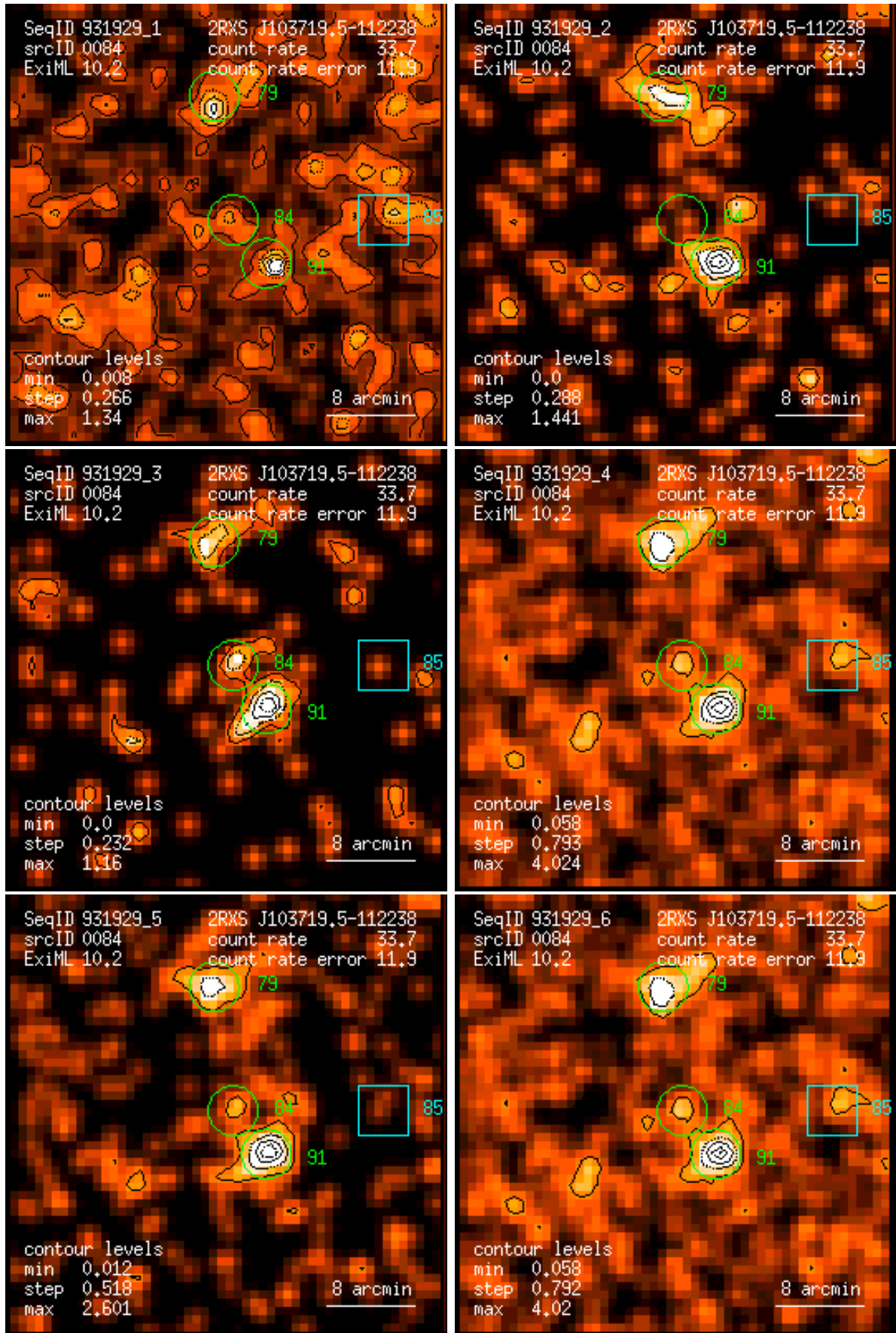
Figure 84: RASS 931929: detection 0084: band rate images, Gaussian filter: (1) PSPC channels 11 – 41, (2) 52 – 90, (3) 91 – 201, (4) 11 – 235, (5) 52 – 201, (6) 11 – 201. Broad band rates in counts/ks. Band rate contour levels in counts/ks/arcmin 2 .
