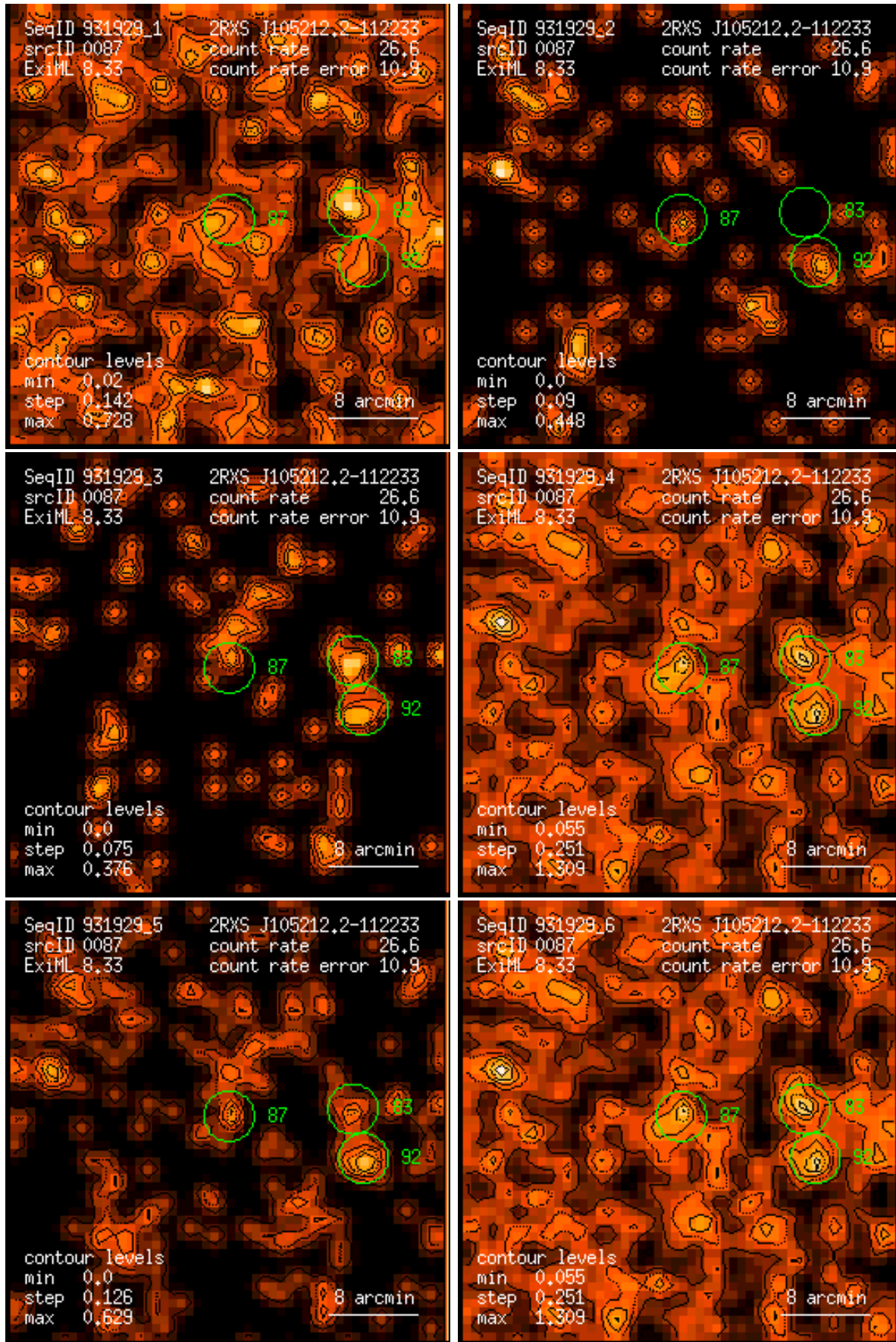
Figure 87: RASS 931929: detection 0087: band rate images, Gaussian filter: (1) PSPC channels 11 – 41, (2) 52 – 90, (3) 91 – 201, (4) 11 – 235, (5) 52 – 201, (6) 11 – 201. Broad band rates in counts/ks. Band rate contour levels in counts/ks/arcmin 2 .
