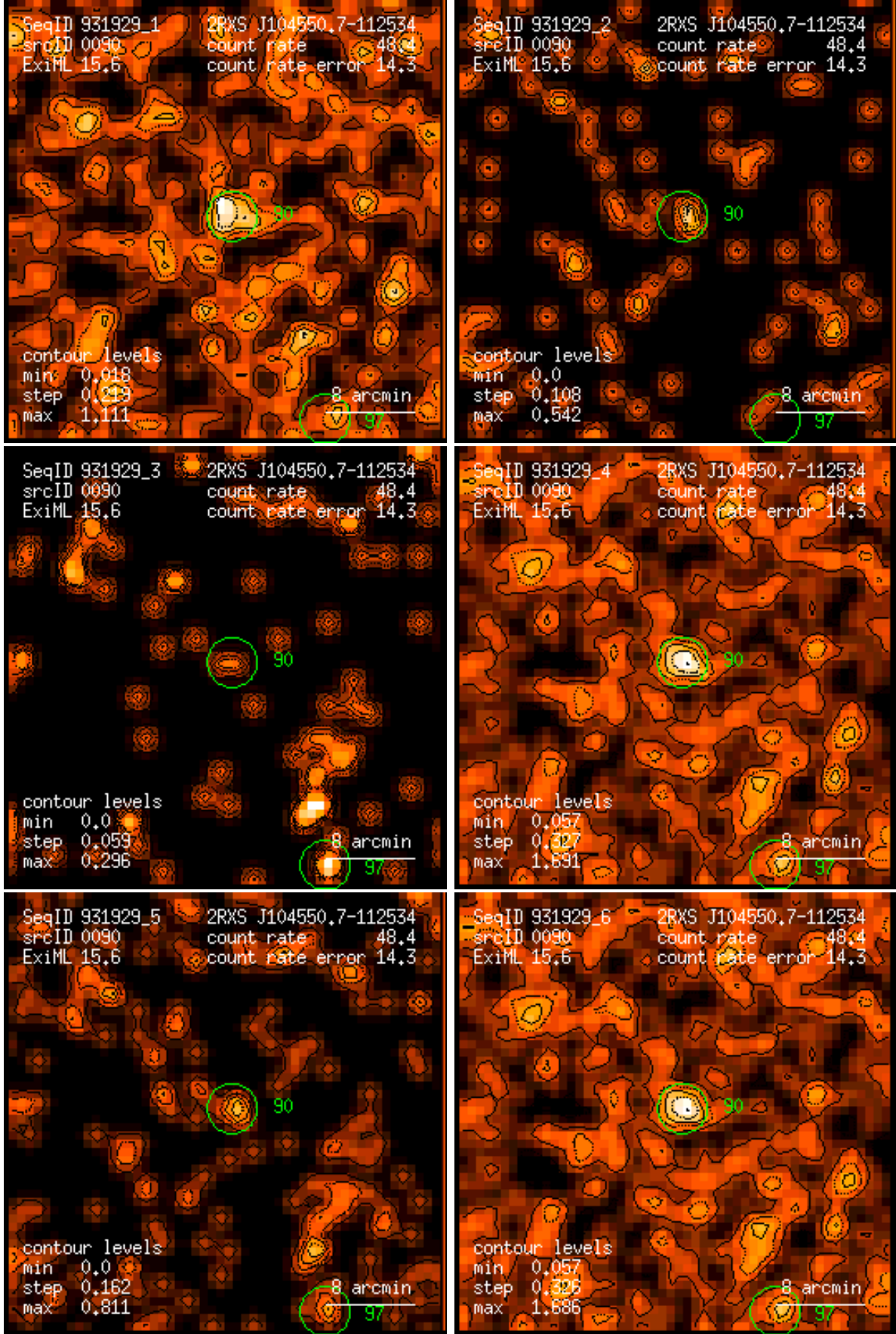
Figure 90: RASS 931929: detection 0090: band rate images, Gaussian filter: (1) PSPC channels 11 – 41, (2) 52 – 90, (3) 91 – 201, (4) 11 – 235, (5) 52 – 201, (6) 11 – 201. Broad band rates in counts/ks. Band rate contour levels in counts/ks/arcmin 2 .
