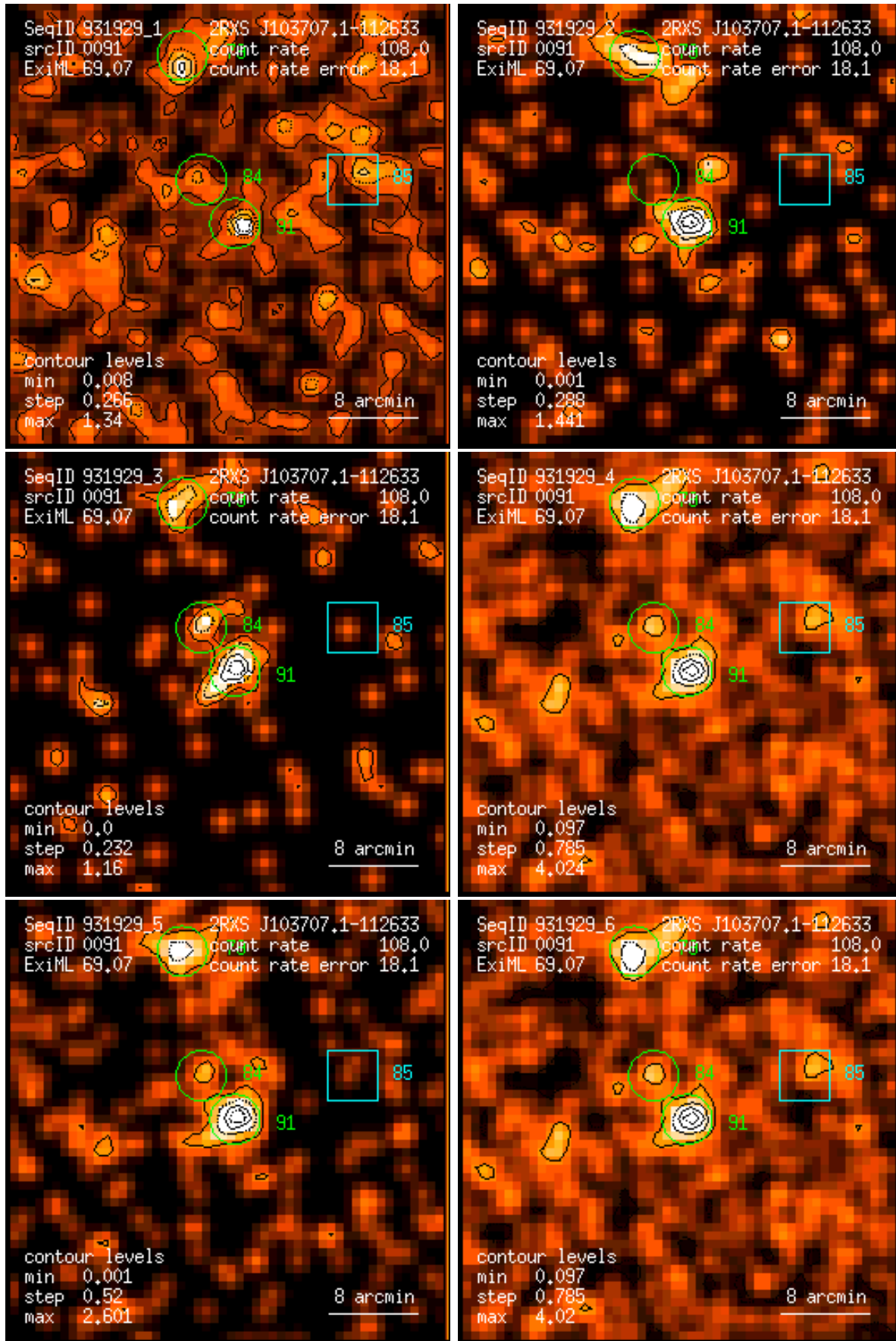
Figure 91: RASS 931929: detection 0091: band rate images, Gaussian filter: (1) PSPC channels 11 – 41, (2) 52 – 90, (3) 91 – 201, (4) 11 – 235, (5) 52 – 201, (6) 11 – 201. Broad band rates in counts/ks. Band rate contour levels in counts/ks/arcmin 2 .
