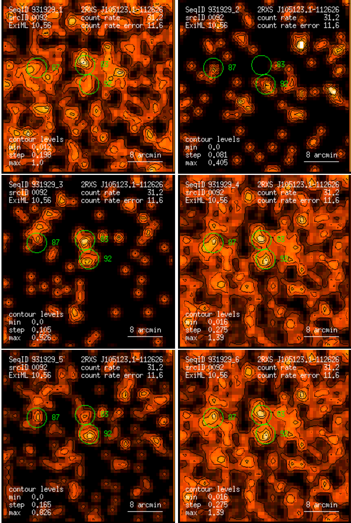
Figure 92: RASS 931929: detection 0092: band rate images, Gaussian filter: (1) PSPC channels 11 – 41, (2) 52 – 90, (3) 91 – 201, (4) 11 – 235, (5) 52 – 201, (6) 11 – 201. Broad band rates in counts/ks. Band rate contour levels in counts/ks/arcmin 2 .
