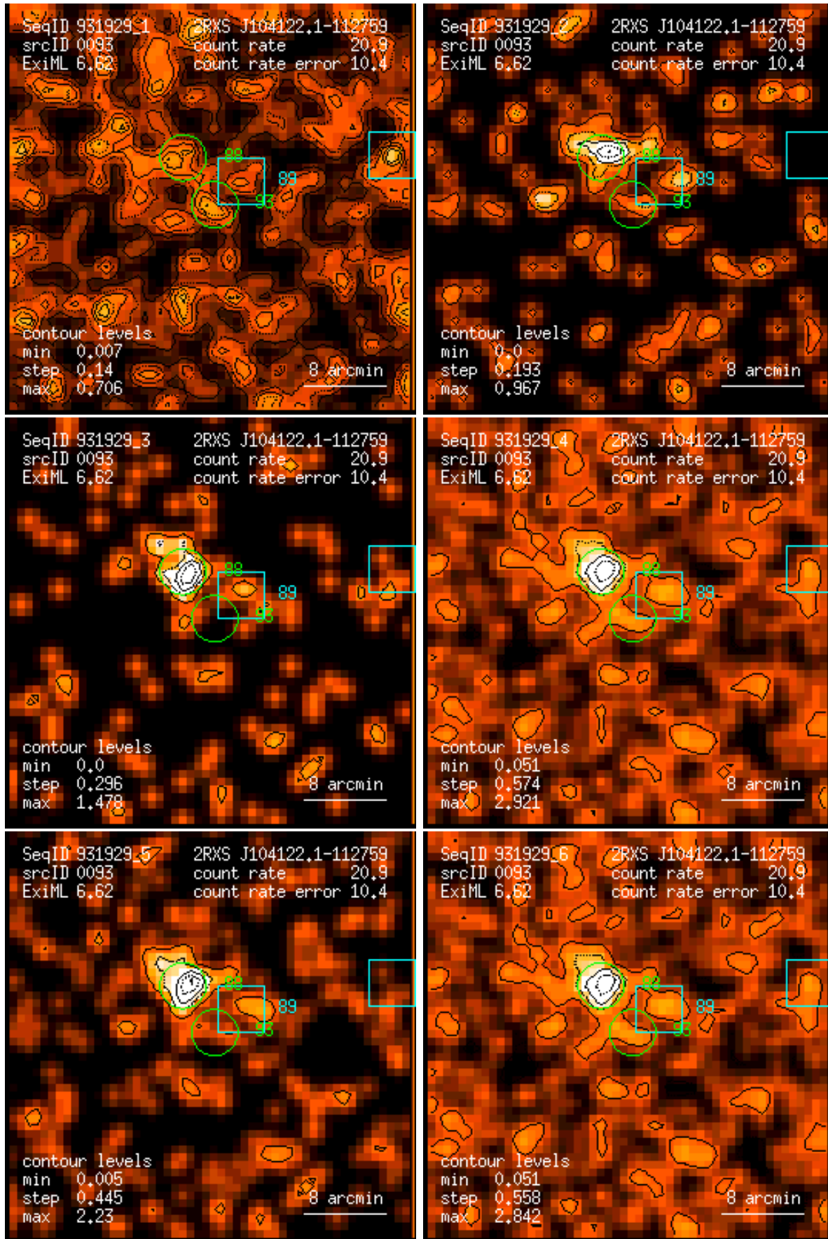
Figure 93: RASS 931929: detection 0093: band rate images, Gaussian filter: (1) PSPC channels 11 – 41, (2) 52 – 90, (3) 91 – 201, (4) 11 – 235, (5) 52 – 201, (6) 11 – 201. Broad band rates in counts/ks. Band rate contour levels in counts/ks/arcmin 2 .
