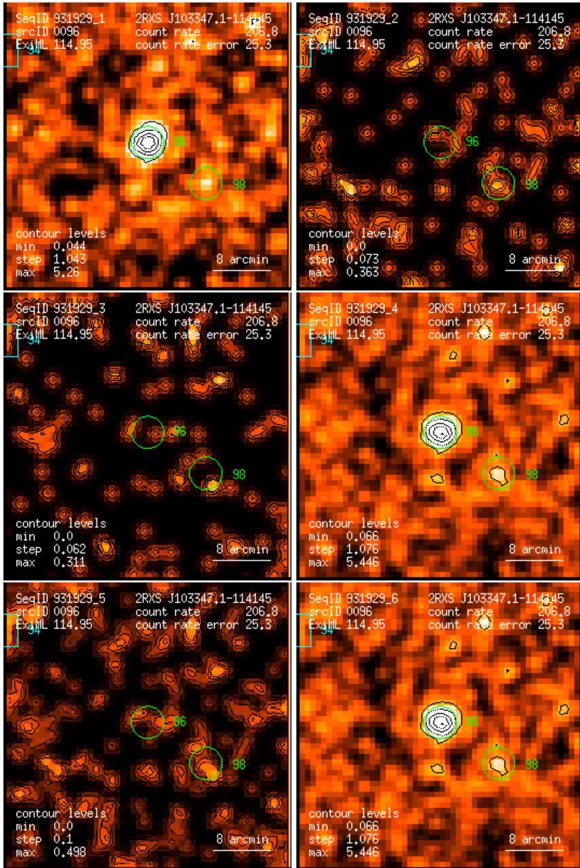
Figure 96: RASS 931929: detection 0096: band rate images, Gaussian filter: (1) PSPC channels 11 – 41, (2) 52 – 90, (3) 91 – 201, (4) 11 – 235, (5) 52 – 201, (6) 11 – 201. Broad band rates in counts/ks. Band rate contour levels in counts/ks/arcmin 2 .
