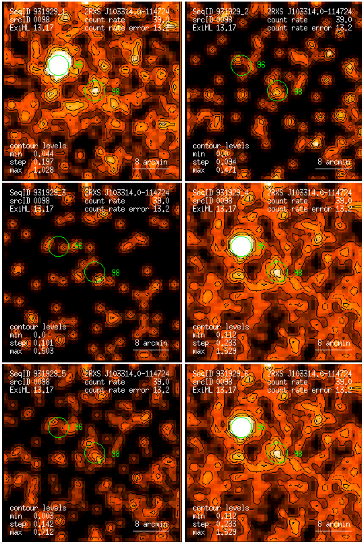
Figure 98: RASS 931929: detection 0098: band rate images, Gaussian filter: (1) PSPC channels 11 – 41, (2) 52 – 90, (3) 91 – 201, (4) 11 – 235, (5) 52 – 201, (6) 11 – 201. Broad band rates in counts/ks. Band rate contour levels in counts/ks/arcmin 2 .
