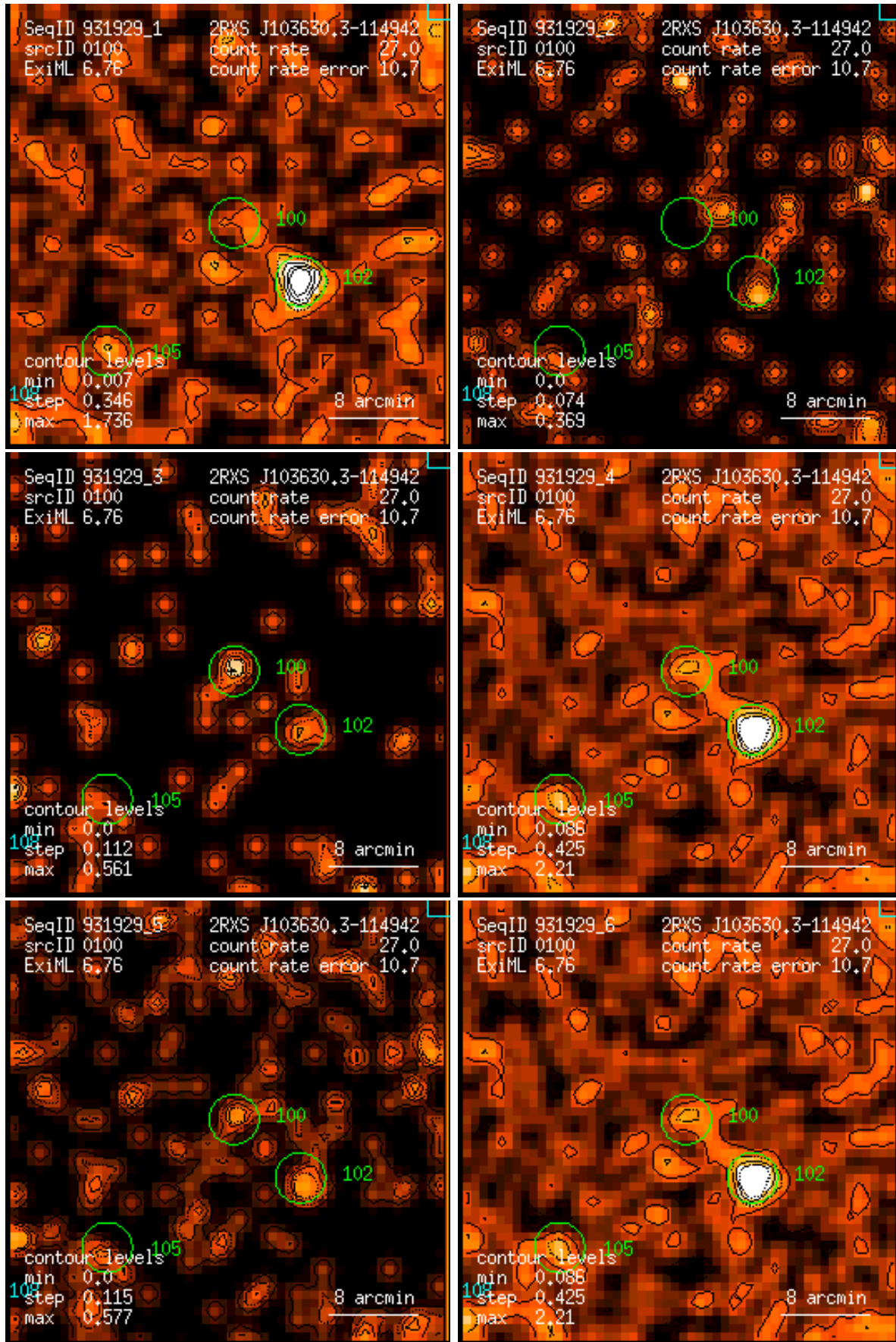
Figure 100: RASS 931929: detection 0100: band rate images, Gaussian filter: (1) PSPC channels 11 – 41, (2) 52 – 90, (3) 91 – 201, (4) 11 – 235, (5) 52 – 201, (6) 11 – 201. Broad band rates in counts/ks. Band rate contour levels in counts/ks/arcmin 2 .
