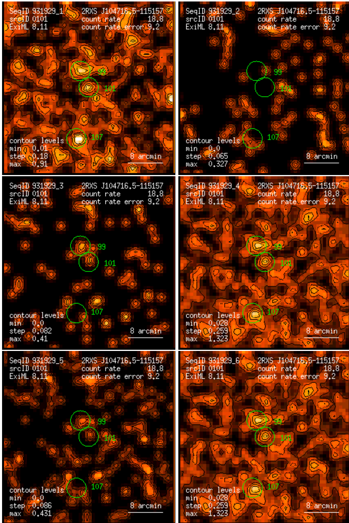
Figure 101: RASS 931929: detection 0101: band rate images, Gaussian filter: (1) PSPC channels 11 – 41, (2) 52 – 90, (3) 91 – 201, (4) 11 – 235, (5) 52 – 201, (6) 11 – 201. Broad band rates in counts/ks. Band rate contour levels in counts/ks/arcmin 2 .
