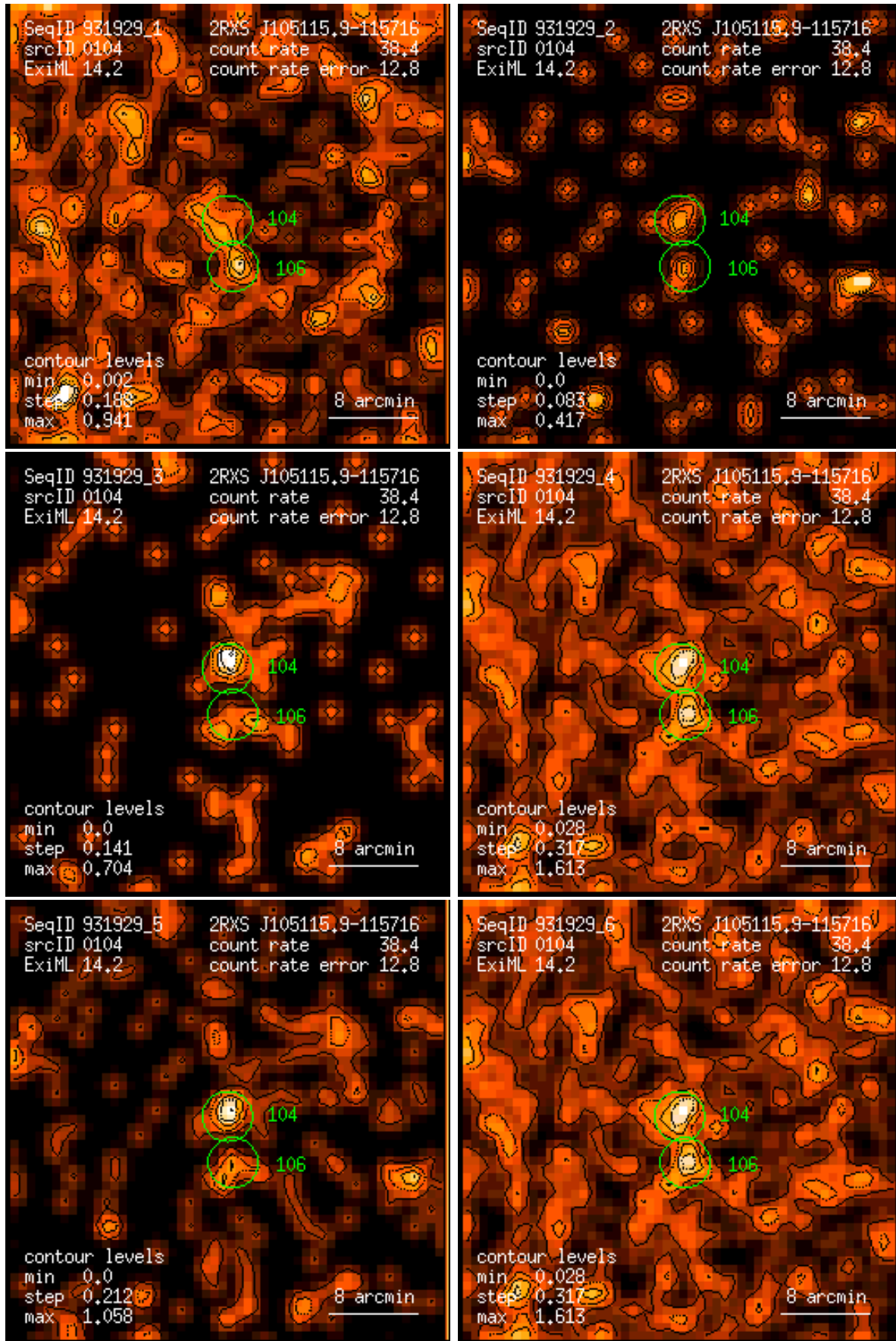
Figure 104: RASS 931929: detection 0104: band rate images, Gaussian filter: (1) PSPC channels 11 – 41, (2) 52 – 90, (3) 91 – 201, (4) 11 – 235, (5) 52 – 201, (6) 11 – 201. Broad band rates in counts/ks. Band rate contour levels in counts/ks/arcmin 2 .
