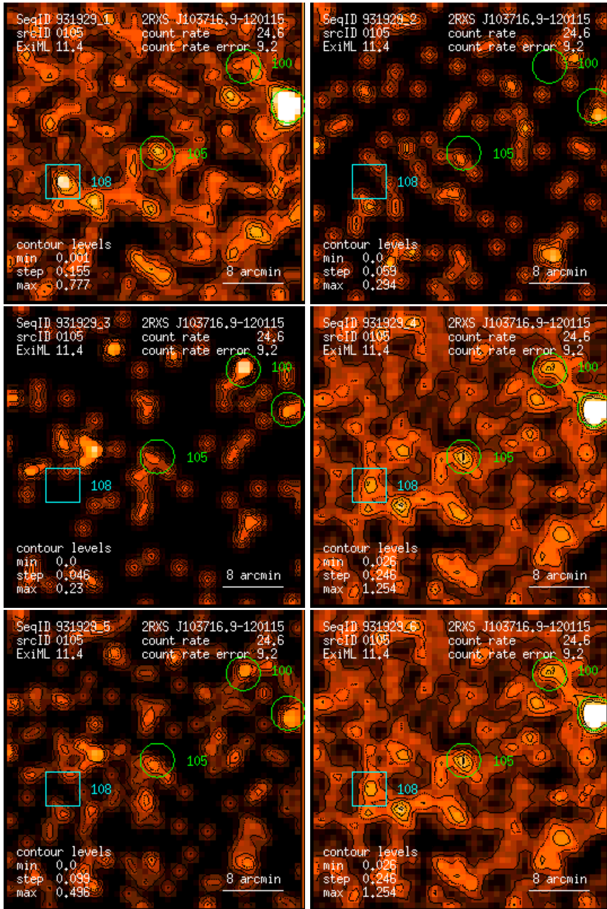
Figure 105: RASS 931929: detection 0105: band rate images, Gaussian filter: (1) PSPC channels 11 – 41, (2) 52 – 90, (3) 91 – 201, (4) 11 – 235, (5) 52 – 201, (6) 11 – 201. Broad band rates in counts/ks. Band rate contour levels in counts/ks/arcmin 2 .
