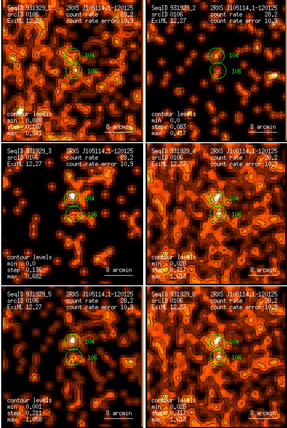
Figure 106: RASS 931929: detection 0106: band rate images, Gaussian filter: (1) PSPC channels 11 – 41, (2) 52 – 90, (3) 91 – 201, (4) 11 – 235, (5) 52 – 201, (6) 11 – 201. Broad band rates in counts/ks. Band rate contour levels in counts/ks/arcmin 2 .
