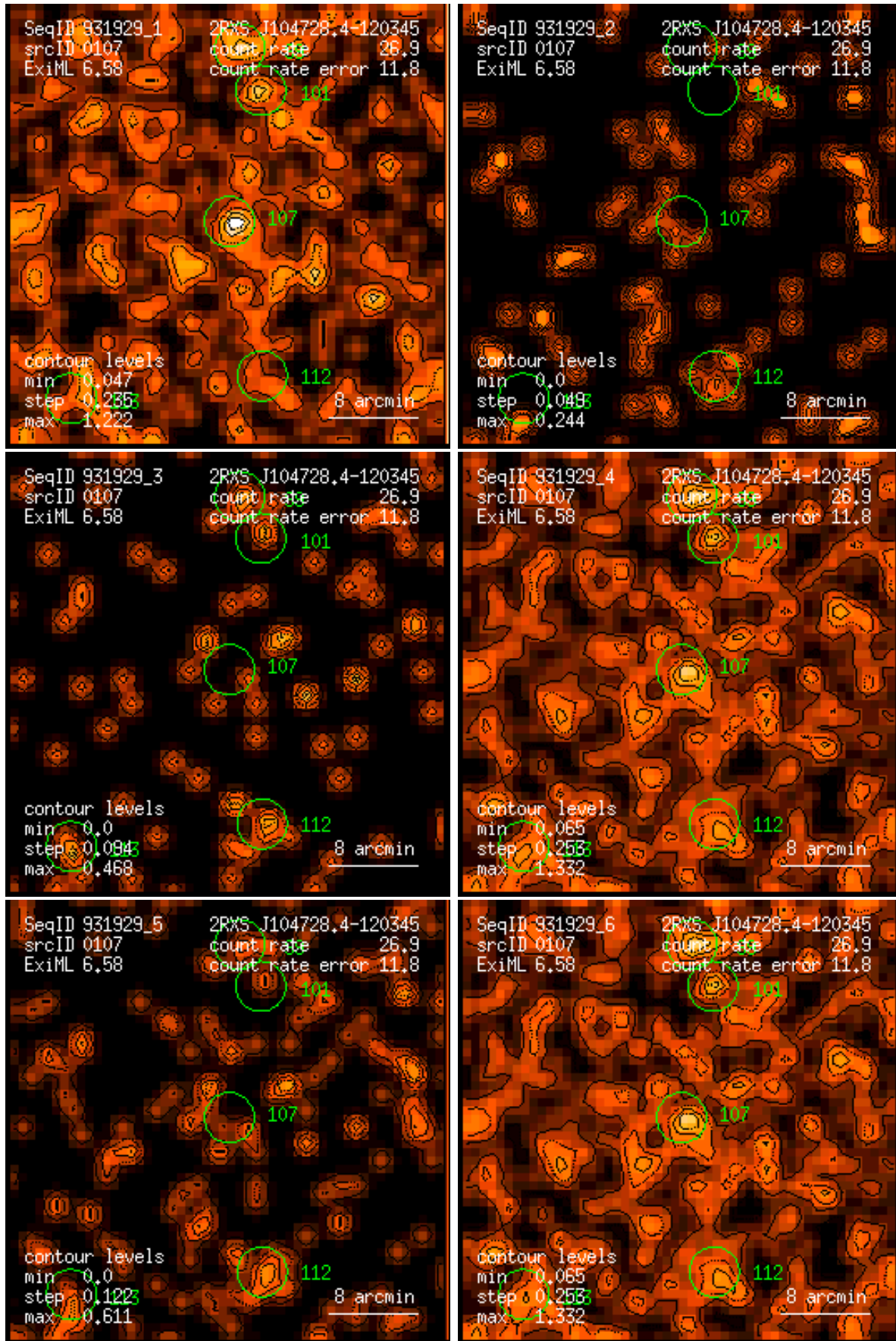
Figure 107: RASS 931929: detection 0107: band rate images, Gaussian filter: (1) PSPC channels 11 – 41, (2) 52 – 90, (3) 91 – 201, (4) 11 – 235, (5) 52 – 201, (6) 11 – 201. Broad band rates in counts/ks. Band rate contour levels in counts/ks/arcmin 2 .
