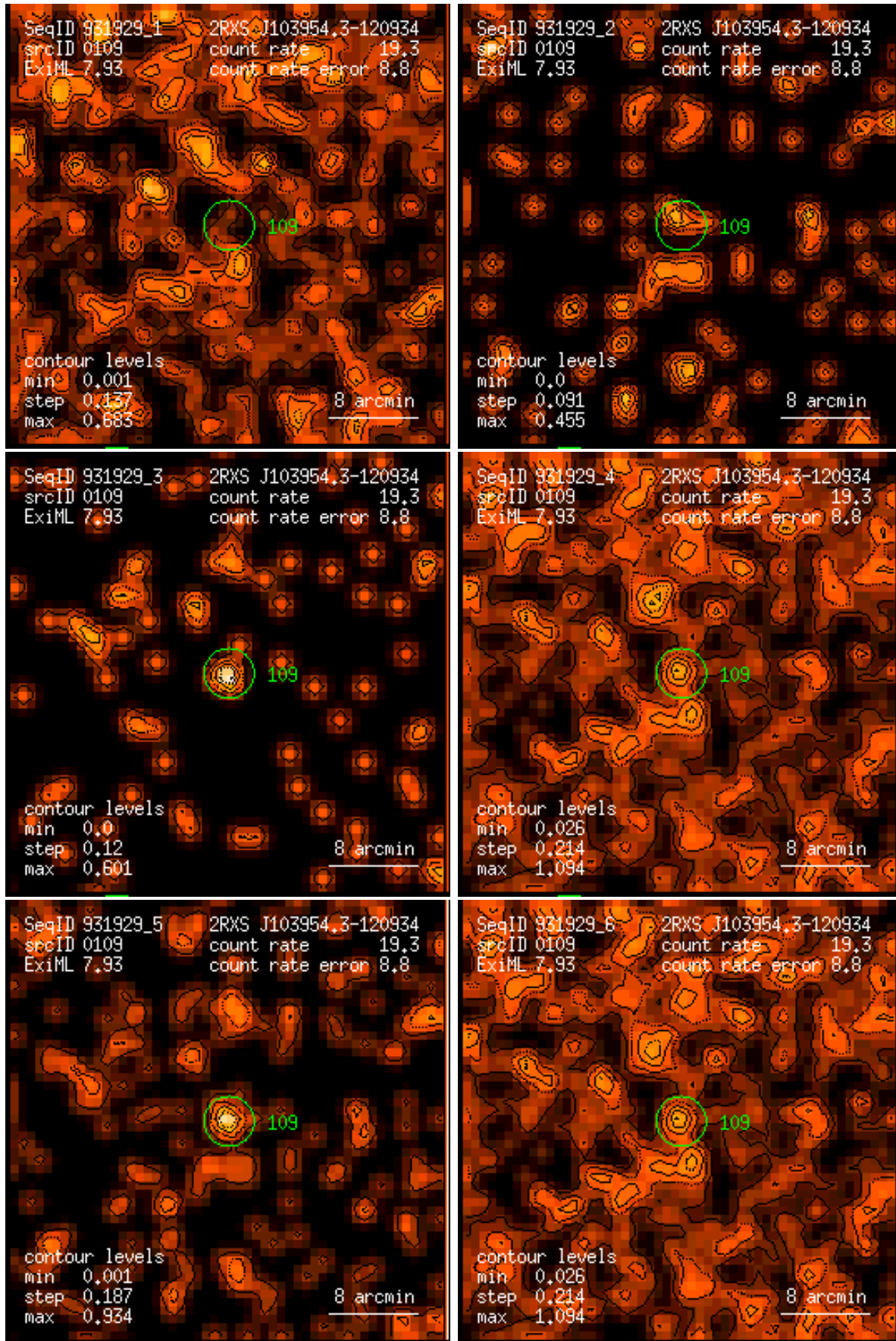
Figure 109: RASS 931929: detection 0109: band rate images, Gaussian filter: (1) PSPC channels 11 – 41, (2) 52 – 90, (3) 91 – 201, (4) 11 – 235, (5) 52 – 201, (6) 11 – 201. Broad band rates in counts/ks. Band rate contour levels in counts/ks/arcmin 2 .
