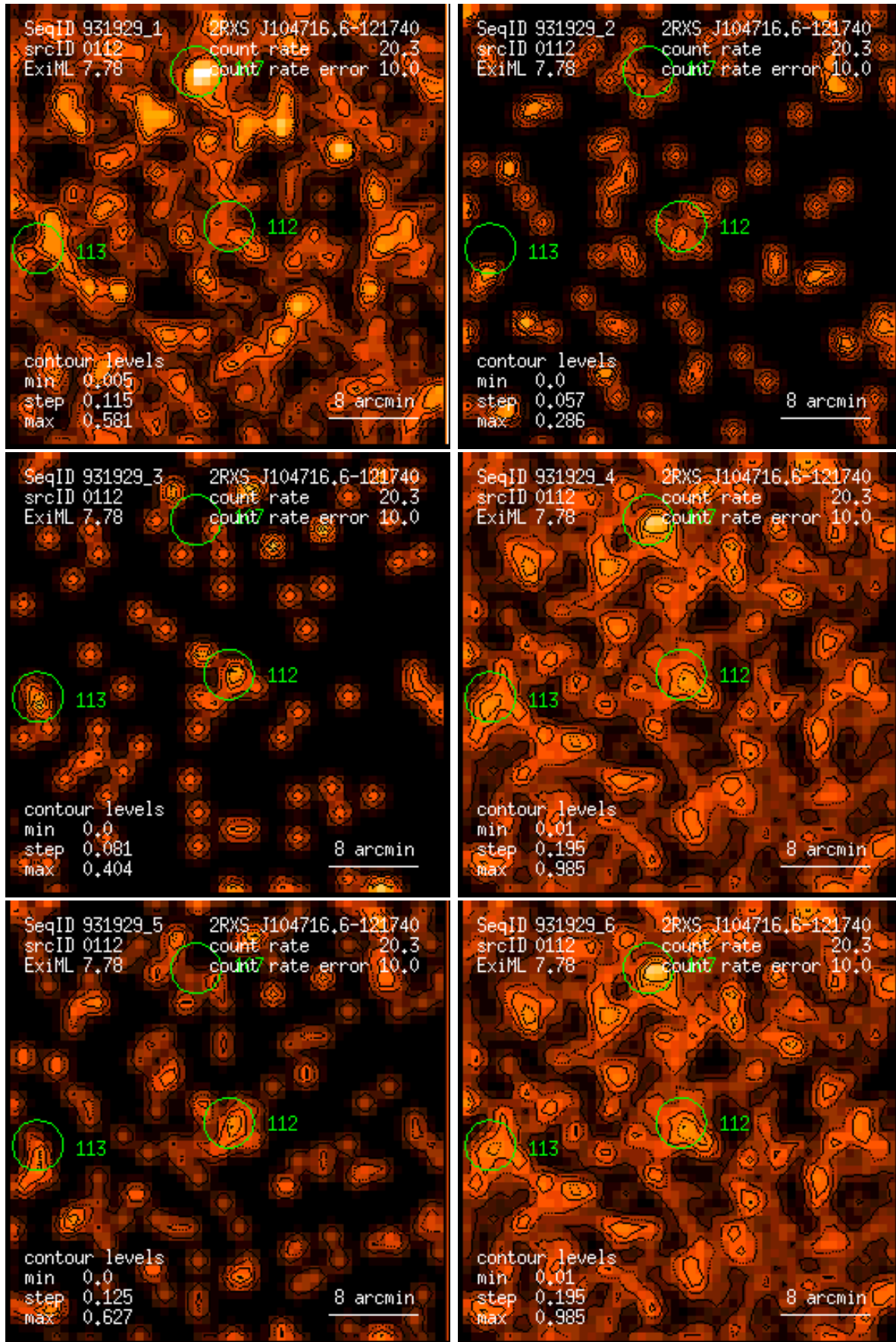
Figure 112: RASS 931929: detection 0112: band rate images, Gaussian filter: (1) PSPC channels 11 – 41, (2) 52 – 90, (3) 91 – 201, (4) 11 – 235, (5) 52 – 201, (6) 11 – 201. Broad band rates in counts/ks. Band rate contour levels in counts/ks/arcmin 2 .
