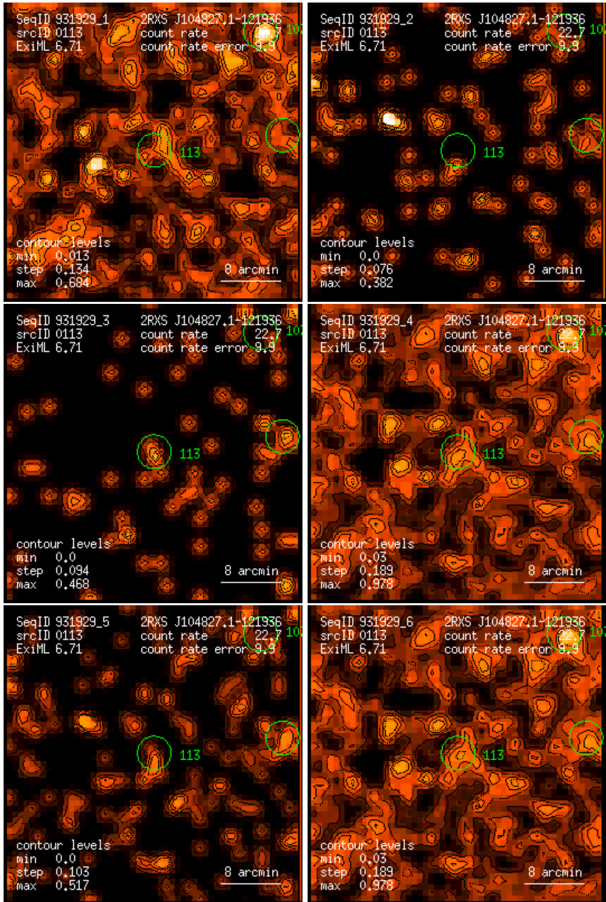
Figure 113: RASS 931929: detection 0113: band rate images, Gaussian filter: (1) PSPC channels 11 – 41, (2) 52 – 90, (3) 91 – 201, (4) 11 – 235, (5) 52 – 201, (6) 11 – 201. Broad band rates in counts/ks. Band rate contour levels in counts/ks/arcmin 2 .
