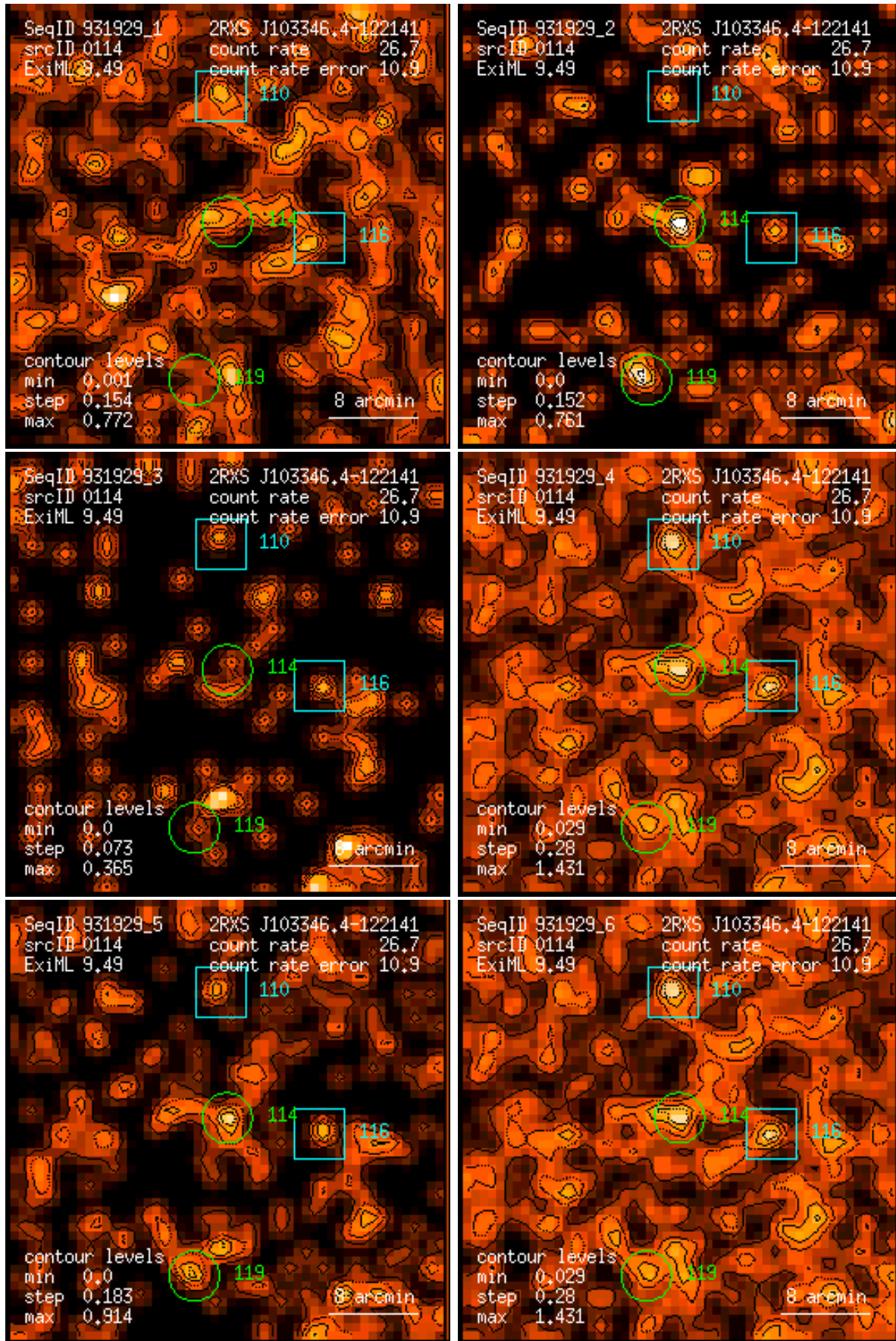
Figure 114: RASS 931929: detection 0114: band rate images, Gaussian filter: (1) PSPC channels 11 – 41, (2) 52 – 90, (3) 91 – 201, (4) 11 – 235, (5) 52 – 201, (6) 11 – 201. Broad band rates in counts/ks. Band rate contour levels in counts/ks/arcmin 2 .
