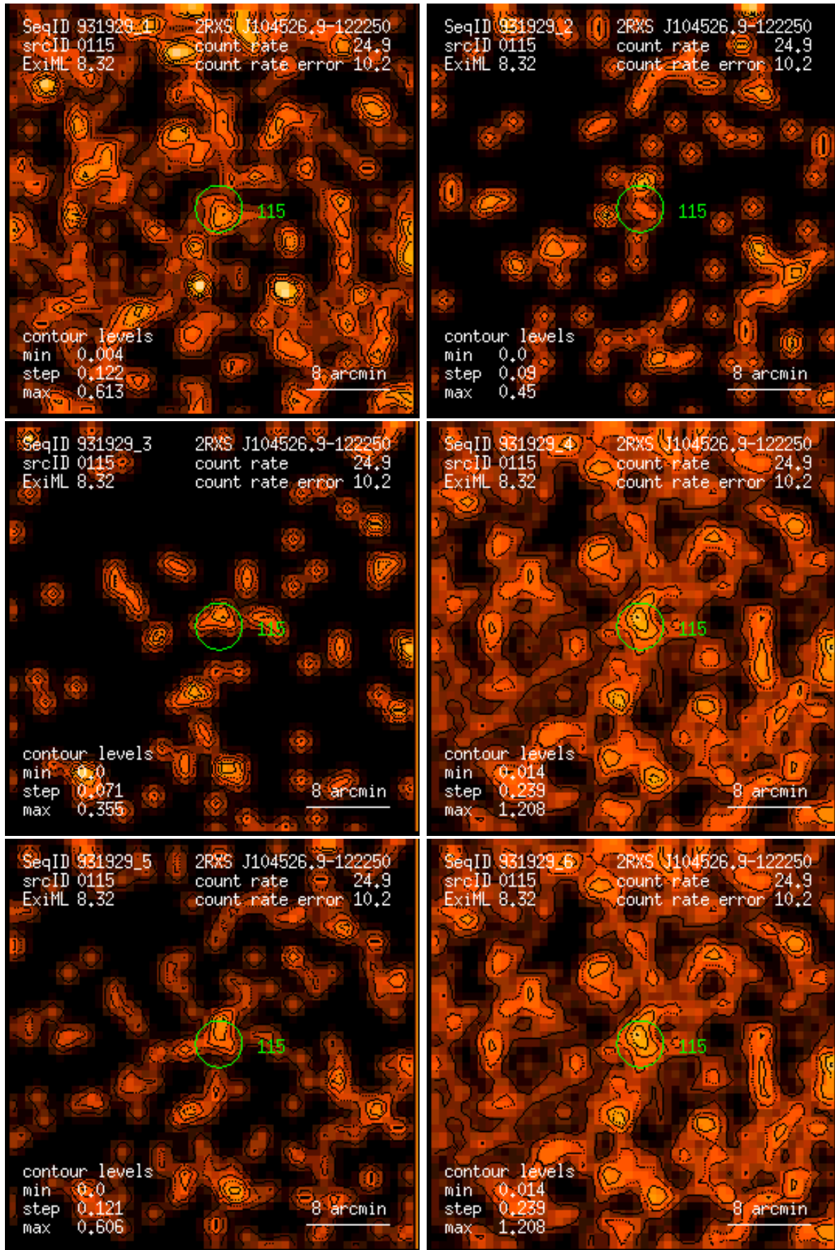
Figure 115: RASS 931929: detection 0115: band rate images, Gaussian filter: (1) PSPC channels 11 – 41, (2) 52 – 90, (3) 91 – 201, (4) 11 – 235, (5) 52 – 201, (6) 11 – 201. Broad band rates in counts/ks. Band rate contour levels in counts/ks/arcmin 2 .
