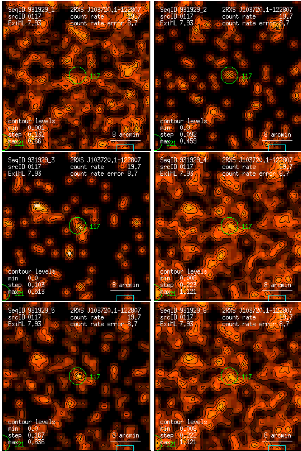
Figure 117: RASS 931929: detection 0117: band rate images, Gaussian filter: (1) PSPC channels 11 – 41, (2) 52 – 90, (3) 91 – 201, (4) 11 – 235, (5) 52 – 201, (6) 11 – 201. Broad band rates in counts/ks. Band rate contour levels in counts/ks/arcmin 2 .
