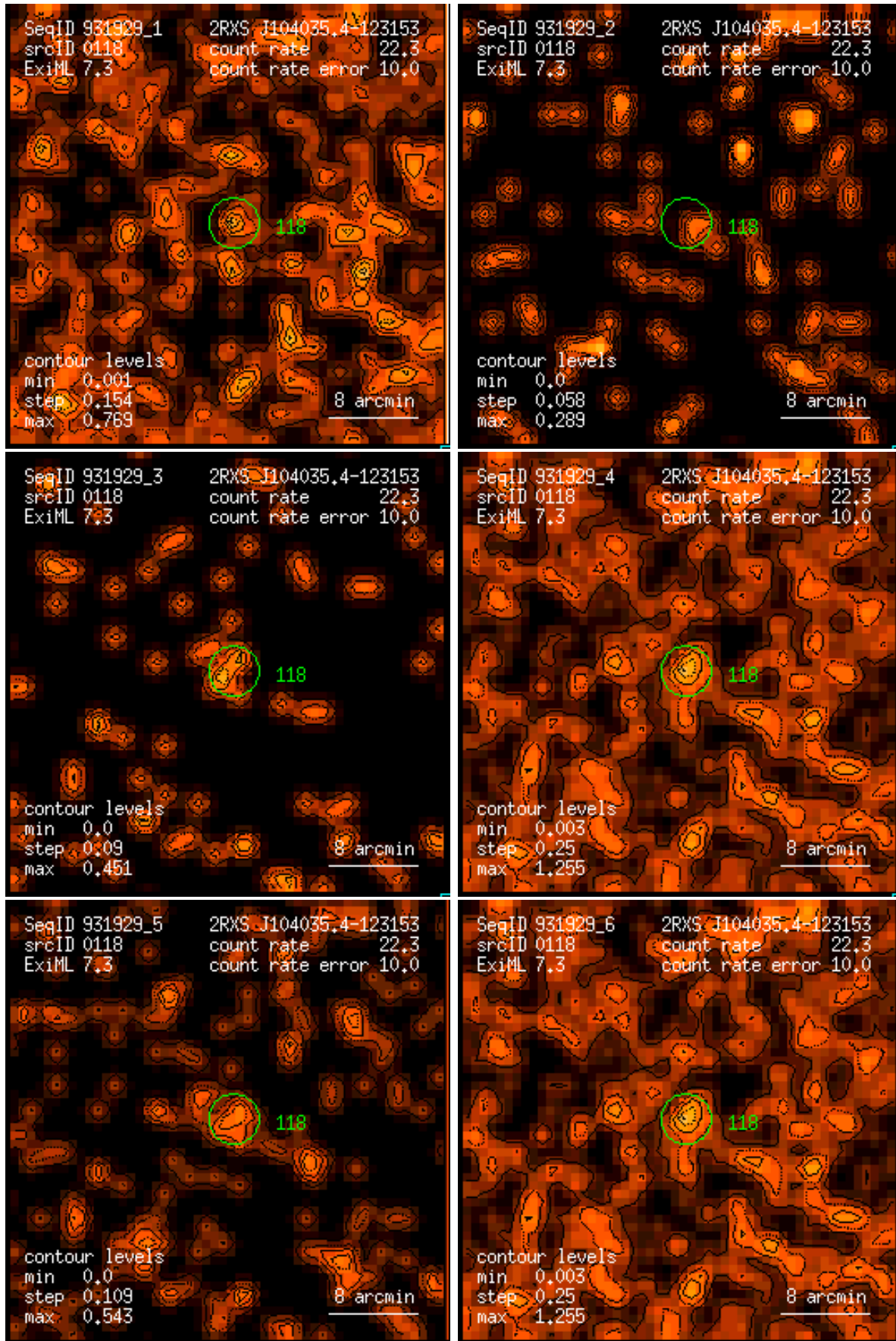
Figure 118: RASS 931929: detection 0118: band rate images, Gaussian filter: (1) PSPC channels 11 – 41, (2) 52 – 90, (3) 91 – 201, (4) 11 – 235, (5) 52 – 201, (6) 11 – 201. Broad band rates in counts/ks. Band rate contour levels in counts/ks/arcmin 2 .
