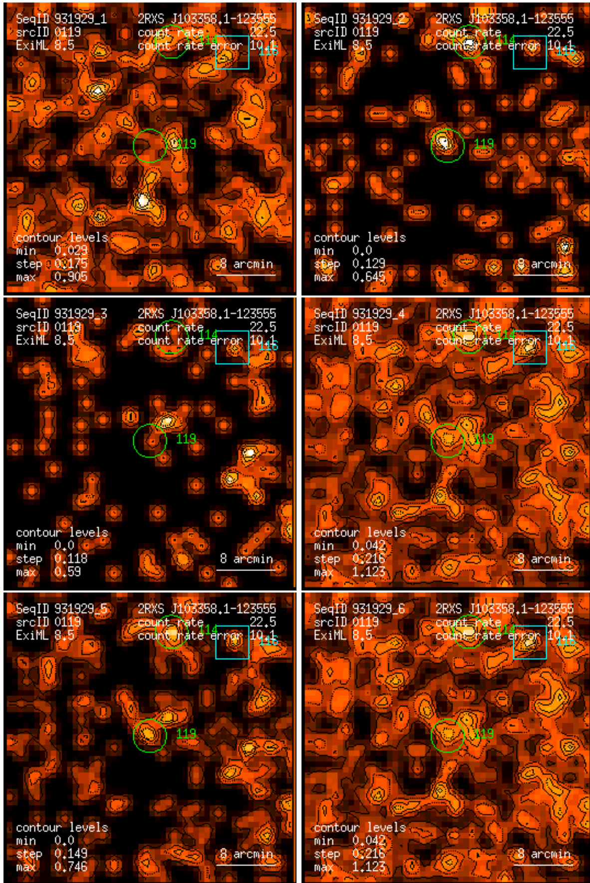
Figure 119: RASS 931929: detection 0119: band rate images, Gaussian filter: (1) PSPC channels 11 – 41, (2) 52 – 90, (3) 91 – 201, (4) 11 – 235, (5) 52 – 201, (6) 11 – 201. Broad band rates in counts/ks. Band rate contour levels in counts/ks/arcmin 2 .
