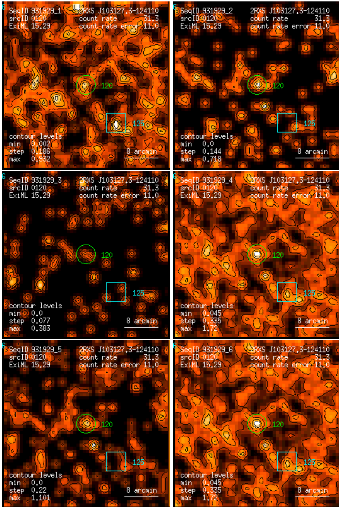
Figure 120: RASS 931929: detection 0120: band rate images, Gaussian filter: (1) PSPC channels 11 – 41, (2) 52 – 90, (3) 91 – 201, (4) 11 – 235, (5) 52 – 201, (6) 11 – 201. Broad band rates in counts/ks. Band rate contour levels in counts/ks/arcmin 2 .
