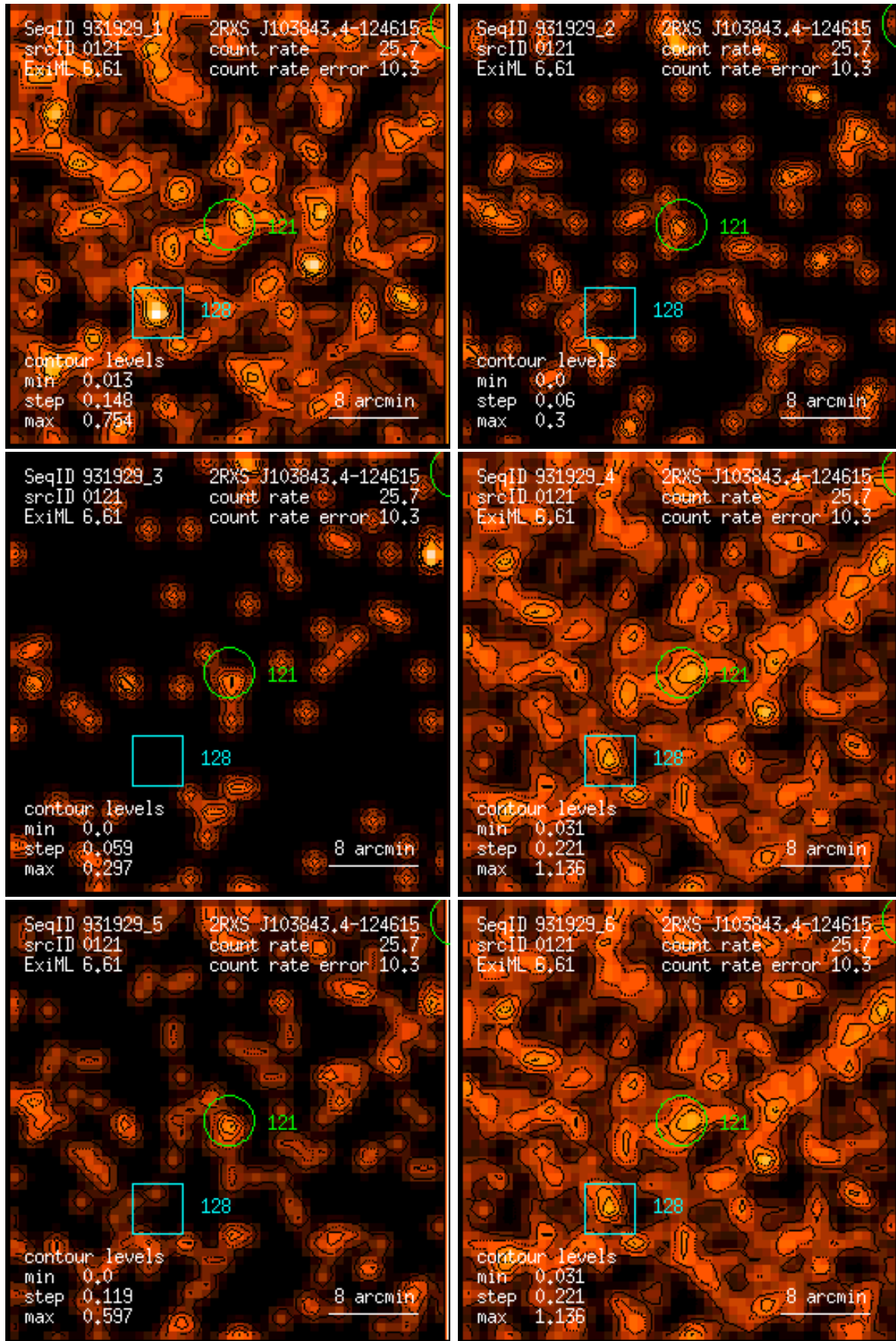
Figure 121: RASS 931929: detection 0121: band rate images, Gaussian filter: (1) PSPC channels 11 – 41, (2) 52 – 90, (3) 91 – 201, (4) 11 – 235, (5) 52 – 201, (6) 11 – 201. Broad band rates in counts/ks. Band rate contour levels in counts/ks/arcmin 2 .
