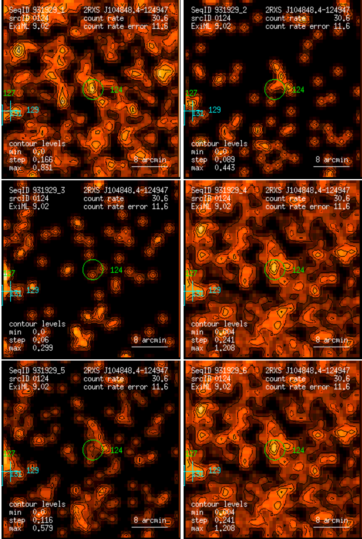
Figure 124: RASS 931929: detection 0124: band rate images, Gaussian filter: (1) PSPC channels 11 – 41, (2) 52 – 90, (3) 91 – 201, (4) 11 – 235, (5) 52 – 201, (6) 11 – 201. Broad band rates in counts/ks. Band rate contour levels in counts/ks/arcmin 2 .
