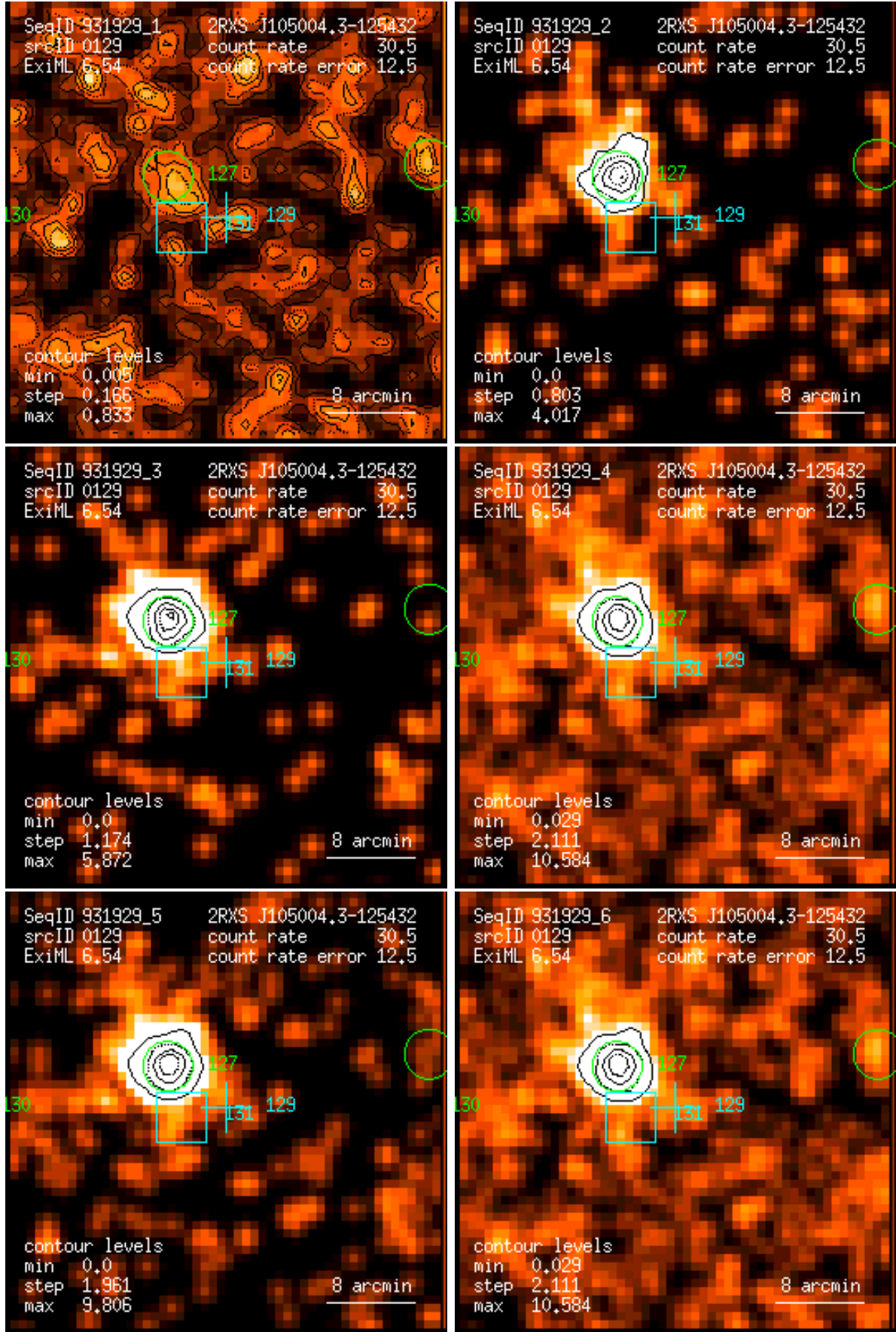
Figure 129: RASS 931929: detection 0129: band rate images, Gaussian filter: (1) PSPC channels 11 – 41, (2) 52 – 90, (3) 91 – 201, (4) 11 – 235, (5) 52 – 201, (6) 11 – 201. Broad band rates in counts/ks. Band rate contour levels in counts/ks/arcmin 2 .
