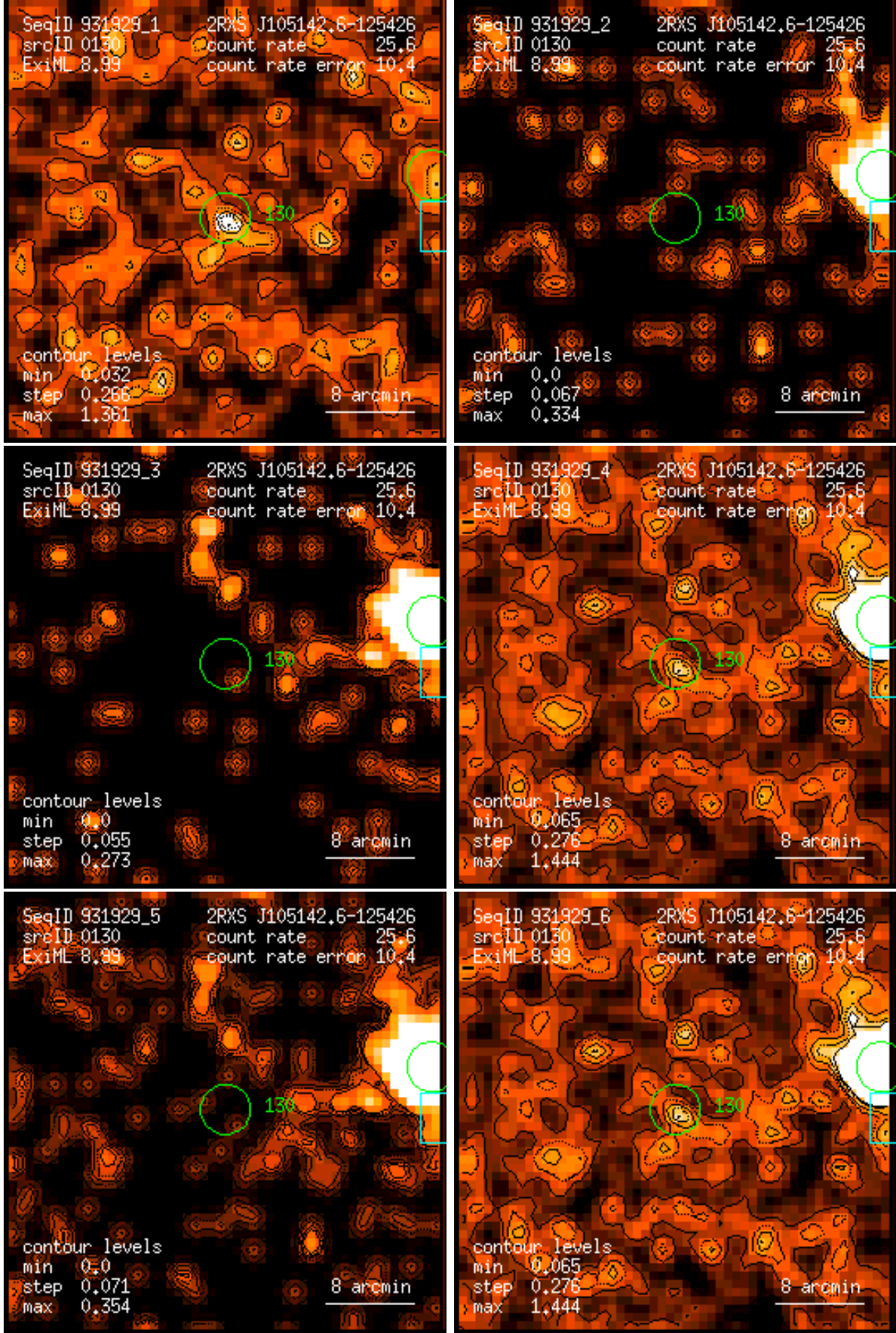
Figure 130: RASS 931929: detection 0130: band rate images, Gaussian filter: (1) PSPC channels 11 – 41, (2) 52 – 90, (3) 91 – 201, (4) 11 – 235, (5) 52 – 201, (6) 11 – 201. Broad band rates in counts/ks. Band rate contour levels in counts/ks/arcmin 2 .
