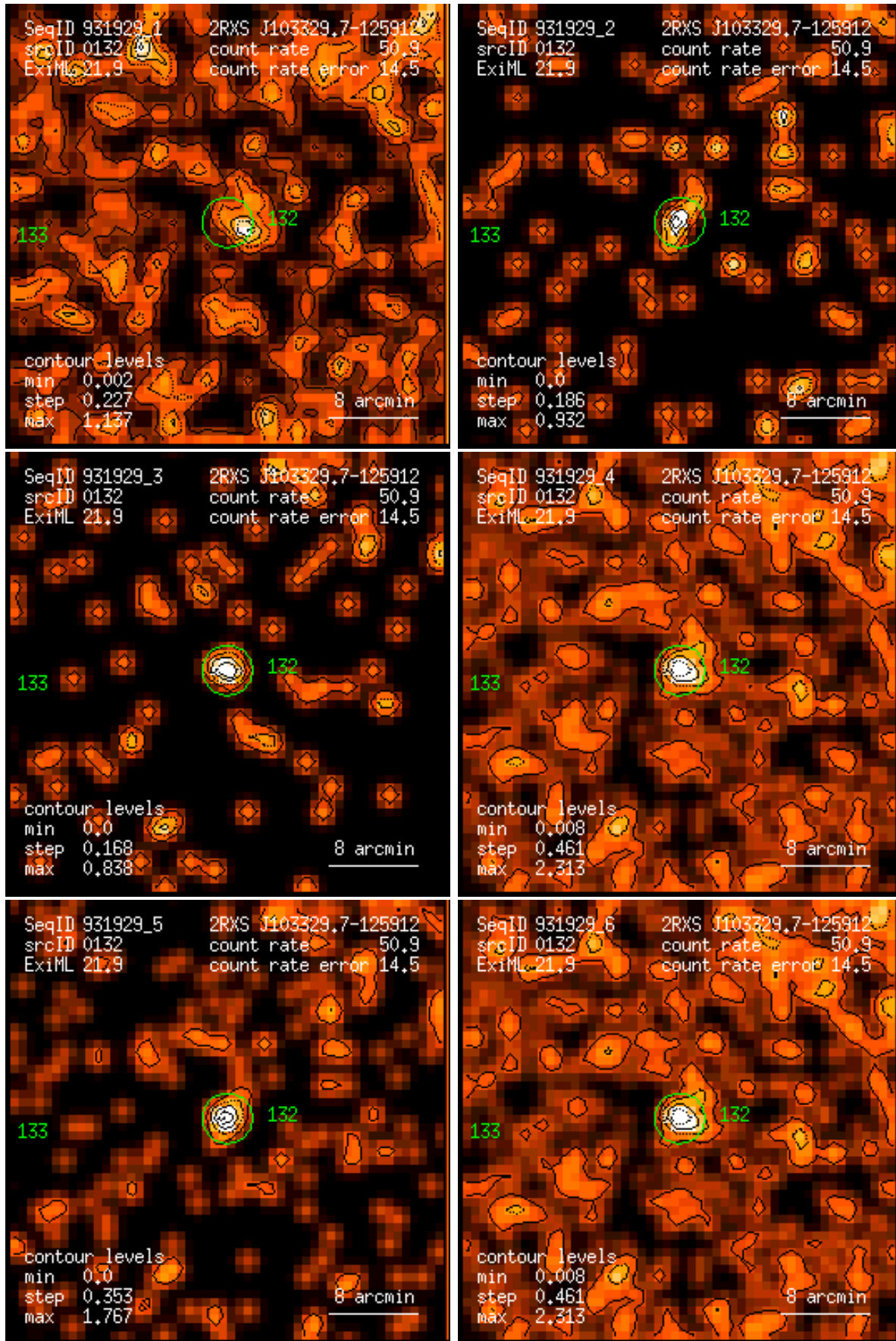
Figure 132: RASS 931929: detection 0132: band rate images, Gaussian filter: (1) PSPC channels 11 – 41, (2) 52 – 90, (3) 91 – 201, (4) 11 – 235, (5) 52 – 201, (6) 11 – 201. Broad band rates in counts/ks. Band rate contour levels in counts/ks/arcmin 2 .
