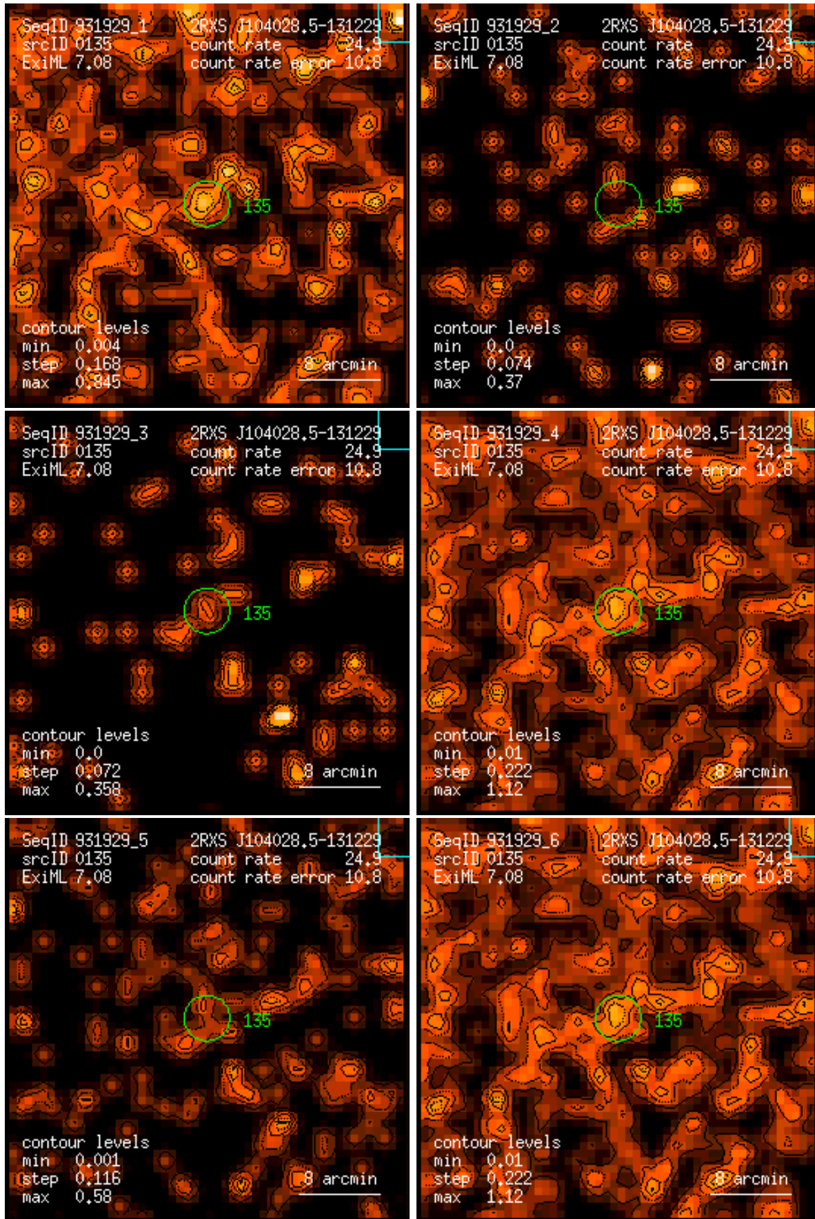
Figure 135: RASS 931929: detection 0135: band rate images, Gaussian filter: (1) PSPC channels 11 – 41, (2) 52 – 90, (3) 91 – 201, (4) 11 – 235, (5) 52 – 201, (6) 11 – 201. Broad band rates in counts/ks. Band rate contour levels in counts/ks/arcmin 2 .
