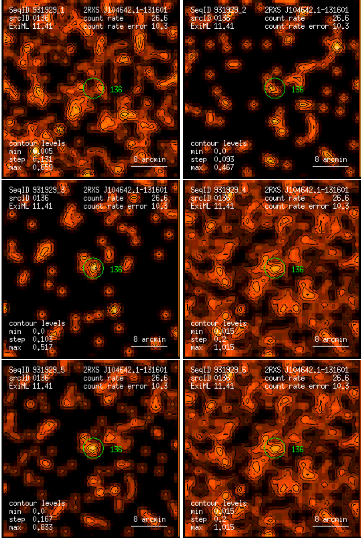
Figure 136: RASS 931929: detection 0136: band rate images, Gaussian filter: (1) PSPC channels 11 – 41, (2) 52 – 90, (3) 91 – 201, (4) 11 – 235, (5) 52 – 201, (6) 11 – 201. Broad band rates in counts/ks. Band rate contour levels in counts/ks/arcmin 2 .
