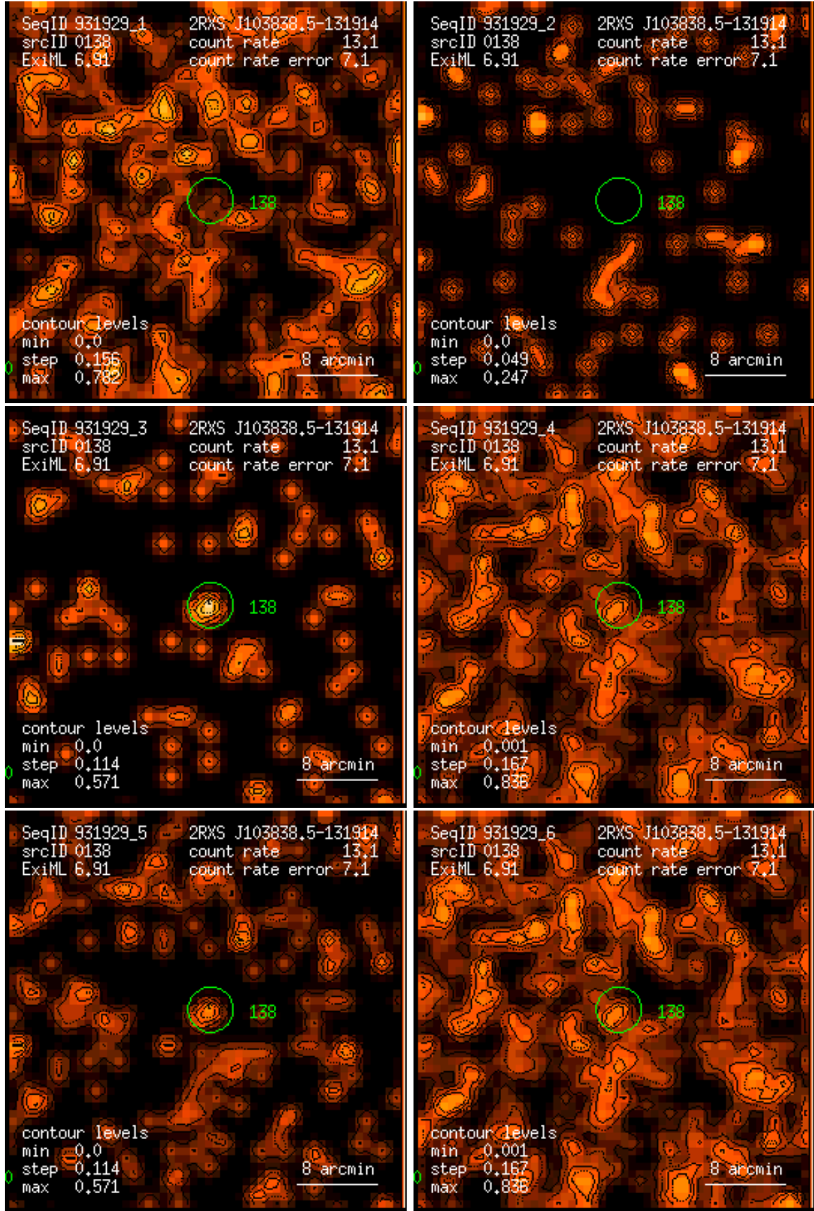
Figure 138: RASS 931929: detection 0138: band rate images, Gaussian filter: (1) PSPC channels 11 – 41, (2) 52 – 90, (3) 91 – 201, (4) 11 – 235, (5) 52 – 201, (6) 11 – 201. Broad band rates in counts/ks. Band rate contour levels in counts/ks/arcmin 2 .
