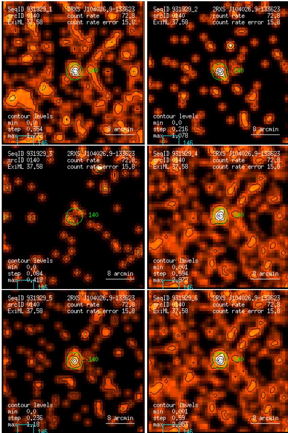
Figure 140: RASS 931929: detection 0140: band rate images, Gaussian filter: (1) PSPC channels 11 – 41, (2) 52 – 90, (3) 91 – 201, (4) 11 – 235, (5) 52 – 201, (6) 11 – 201. Broad band rates in counts/ks. Band rate contour levels in counts/ks/arcmin 2 .
