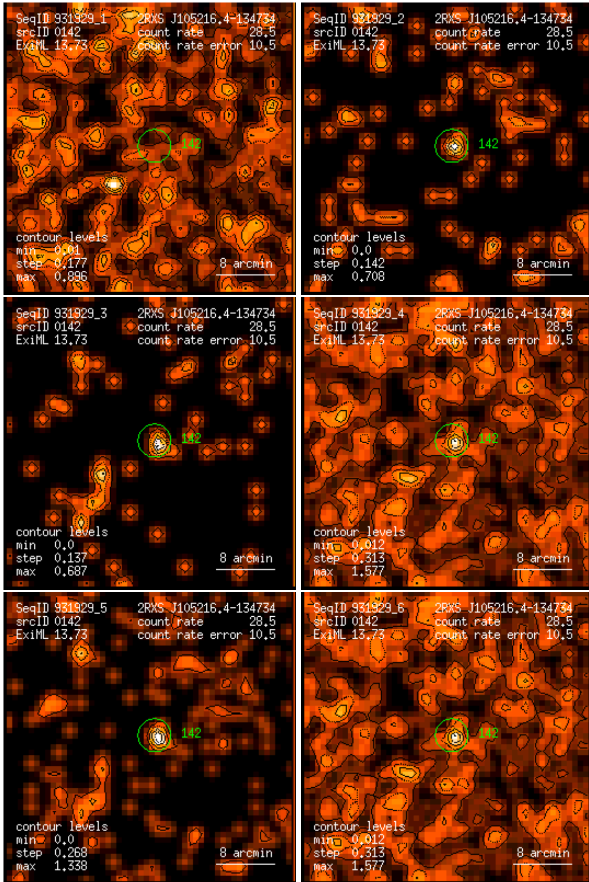
Figure 142: RASS 931929: detection 0142: band rate images, Gaussian filter: (1) PSPC channels 11 – 41, (2) 52 – 90, (3) 91 – 201, (4) 11 – 235, (5) 52 – 201, (6) 11 – 201. Broad band rates in counts/ks. Band rate contour levels in counts/ks/arcmin 2 .
