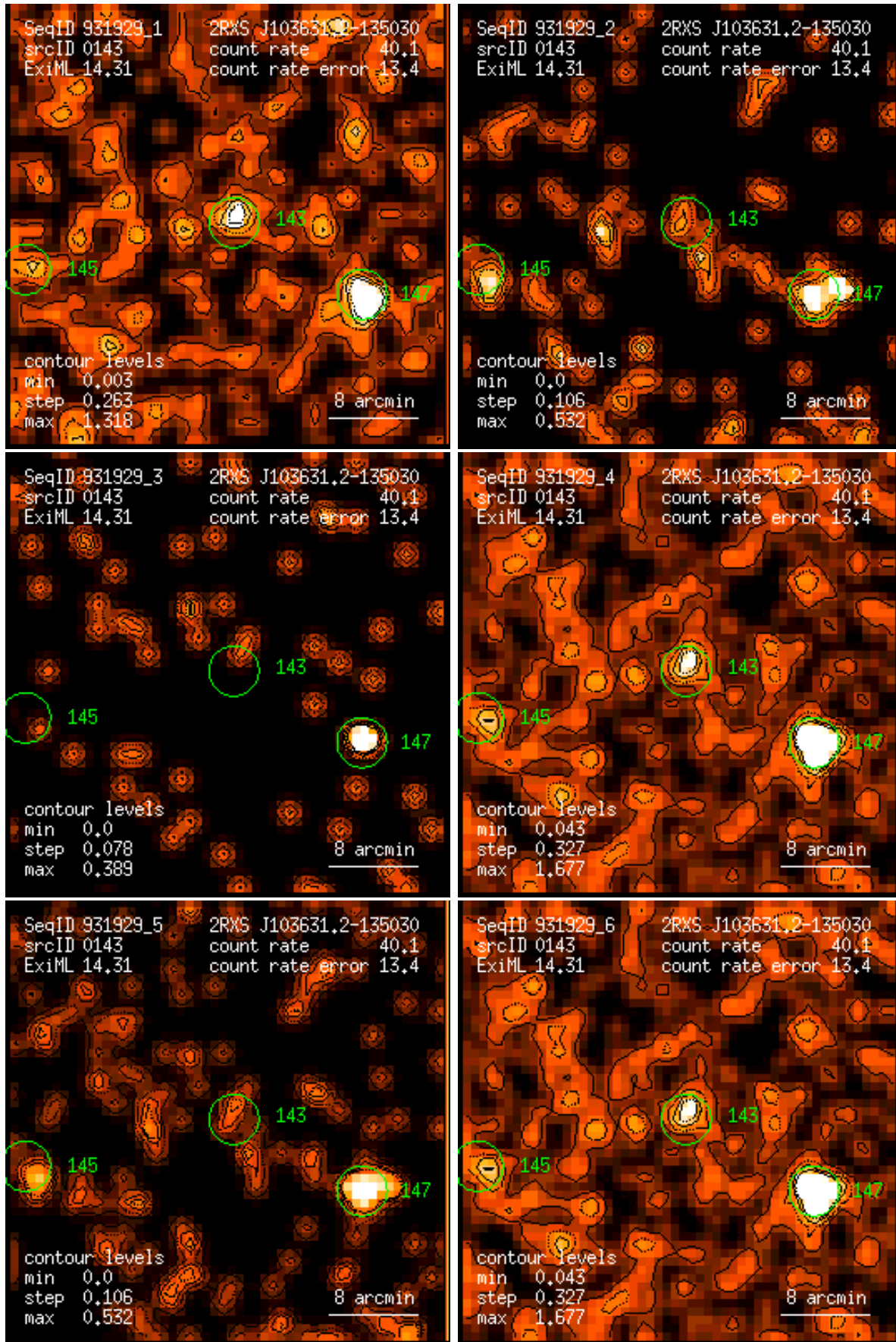
Figure 143: RASS 931929: detection 0143: band rate images, Gaussian filter: (1) PSPC channels 11 – 41, (2) 52 – 90, (3) 91 – 201, (4) 11 – 235, (5) 52 – 201, (6) 11 – 201. Broad band rates in counts/ks. Band rate contour levels in counts/ks/arcmin 2 .
