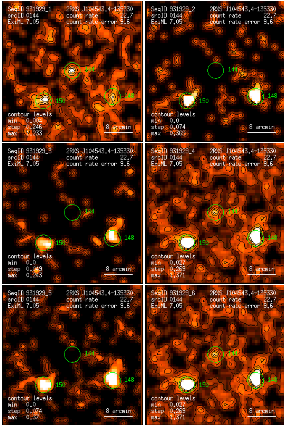
Figure 144: RASS 931929: detection 0144: band rate images, Gaussian filter: (1) PSPC channels 11 – 41, (2) 52 – 90, (3) 91 – 201, (4) 11 – 235, (5) 52 – 201, (6) 11 – 201. Broad band rates in counts/ks. Band rate contour levels in counts/ks/arcmin 2 .
