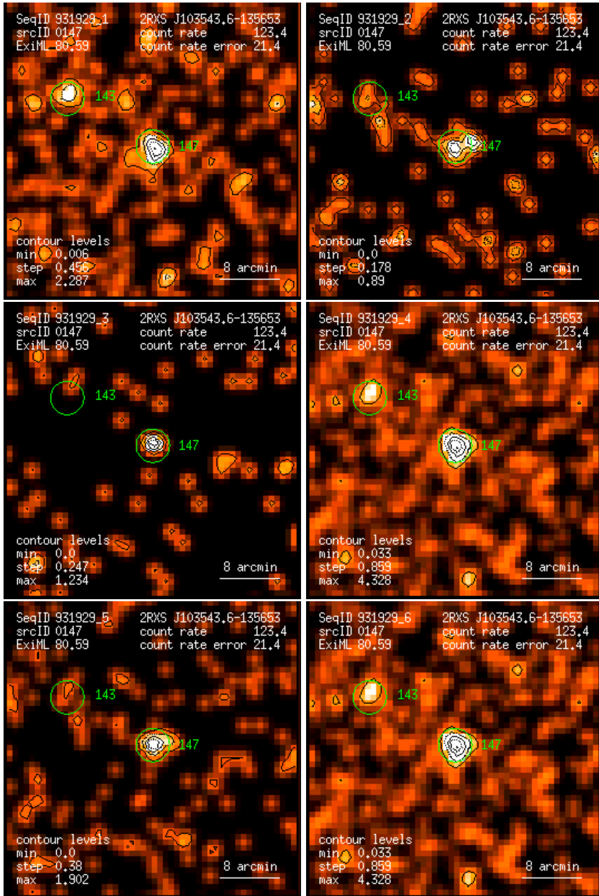
Figure 147: RASS 931929: detection 0147: band rate images, Gaussian filter: (1) PSPC channels 11 – 41, (2) 52 – 90, (3) 91 – 201, (4) 11 – 235, (5) 52 – 201, (6) 11 – 201. Broad band rates in counts/ks. Band rate contour levels in counts/ks/arcmin 2 .
