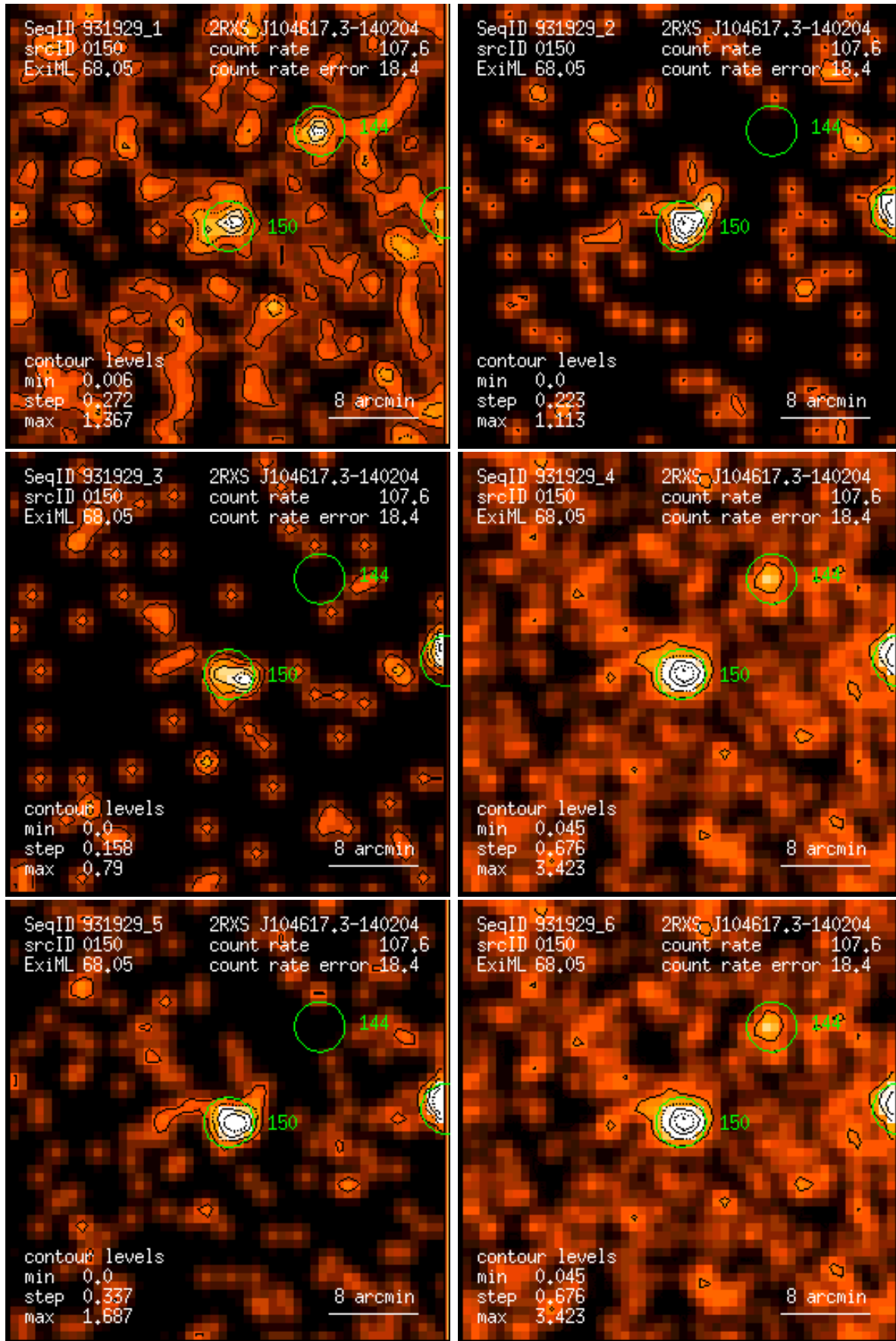
Figure 150: RASS 931929: detection 0150: band rate images, Gaussian filter: (1) PSPC channels 11 – 41, (2) 52 – 90, (3) 91 – 201, (4) 11 – 235, (5) 52 – 201, (6) 11 – 201. Broad band rates in counts/ks. Band rate contour levels in counts/ks/arcmin 2 .
