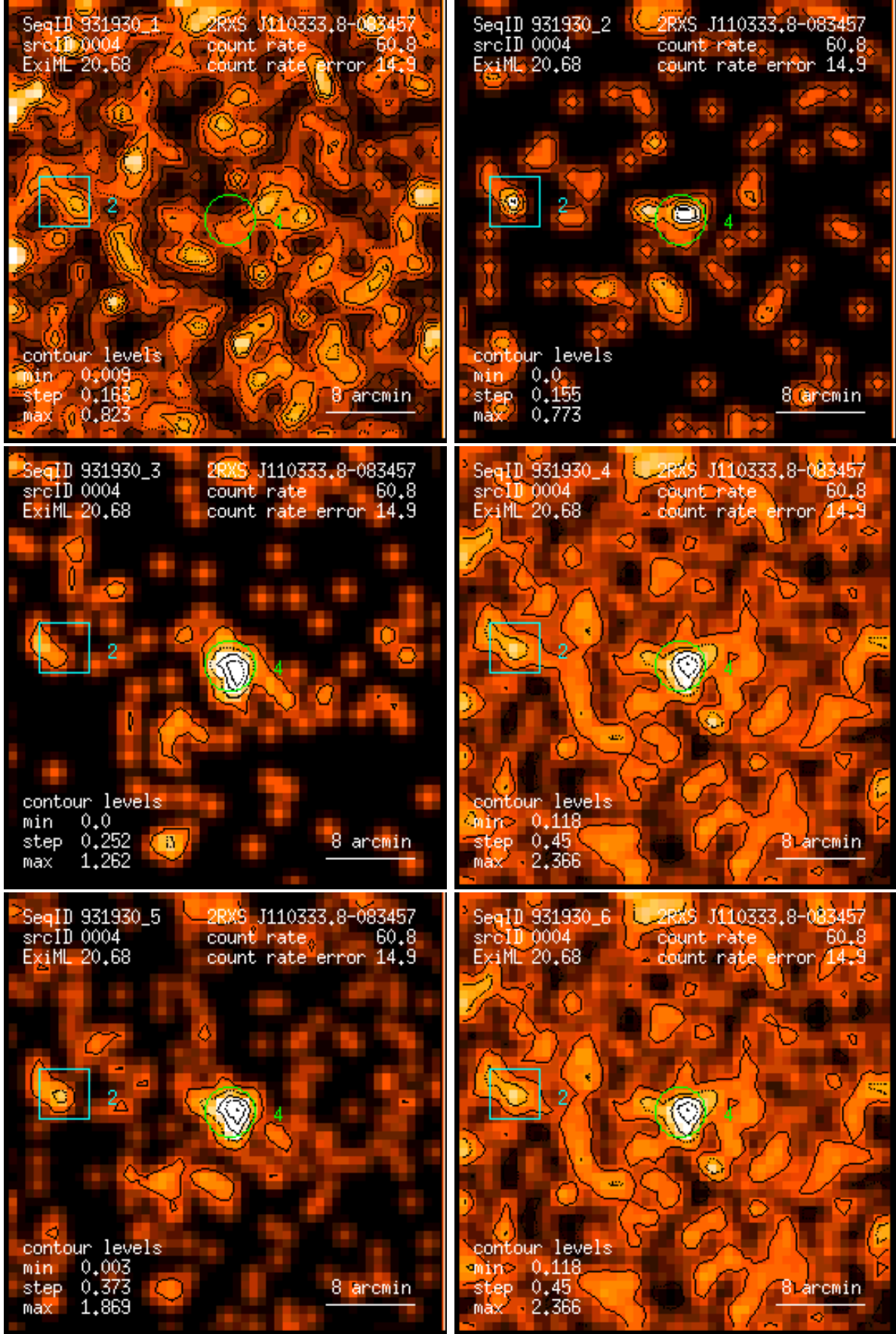
Figure 4: RASS 931930: detection 0004: band rate images, Gaussian filter: (1) PSPC channels 11 – 41, (2) 52 – 90, (3) 91 – 201, (4) 11 – 235, (5) 52 – 201, (6) 11 – 201. Broad band rates in counts/ks. Band rate contour levels in counts/ks/arcmin 2 .
