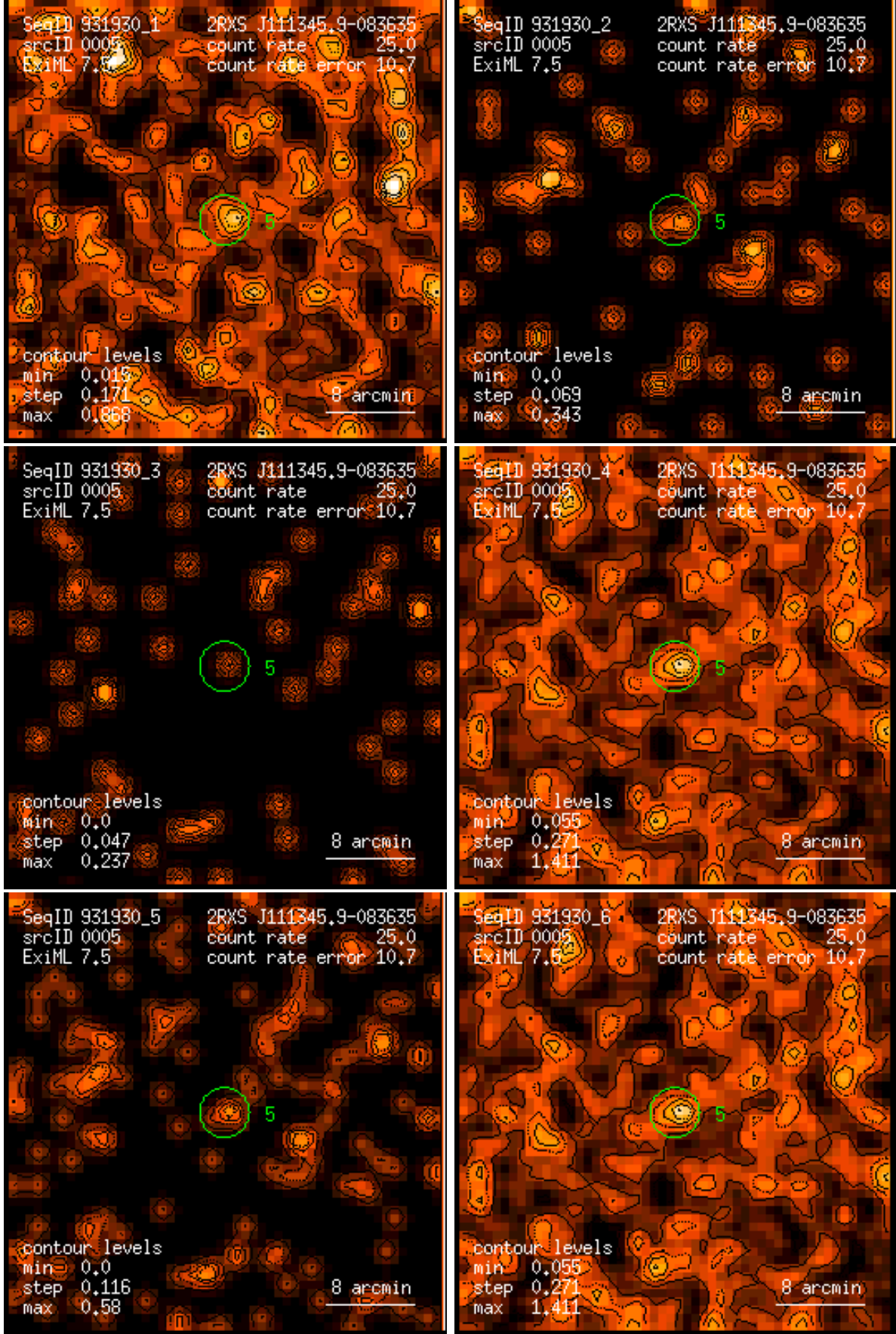
Figure 5: RASS 931930: detection 0005: band rate images, Gaussian filter: (1) PSPC channels 11 – 41, (2) 52 – 90, (3) 91 – 201, (4) 11 – 235, (5) 52 – 201, (6) 11 – 201. Broad band rates in counts/ks. Band rate contour levels in counts/ks/arcmin 2 .
