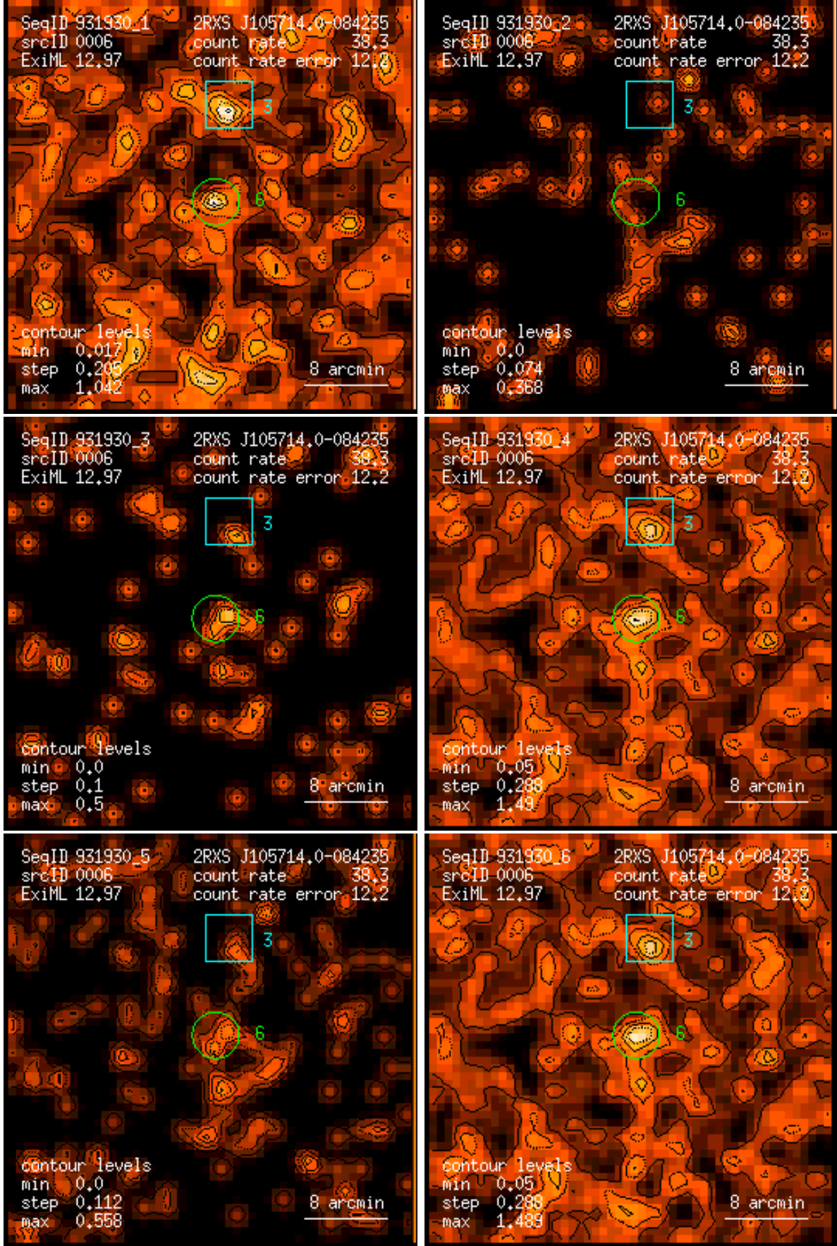
Figure 6: RASS 931930: detection 0006: band rate images, Gaussian filter: (1) PSPC channels 11 – 41, (2) 52 – 90, (3) 91 – 201, (4) 11 – 235, (5) 52 – 201, (6) 11 – 201. Broad band rates in counts/ks. Band rate contour levels in counts/ks/arcmin 2 .
