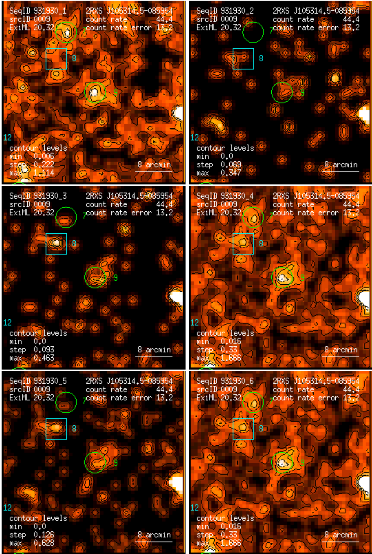
Figure 9: RASS 931930: detection 0009: band rate images, Gaussian filter: (1) PSPC channels 11 – 41, (2) 52 – 90, (3) 91 – 201, (4) 11 – 235, (5) 52 – 201, (6) 11 – 201. Broad band rates in counts/ks. Band rate contour levels in counts/ks/arcmin 2 .
