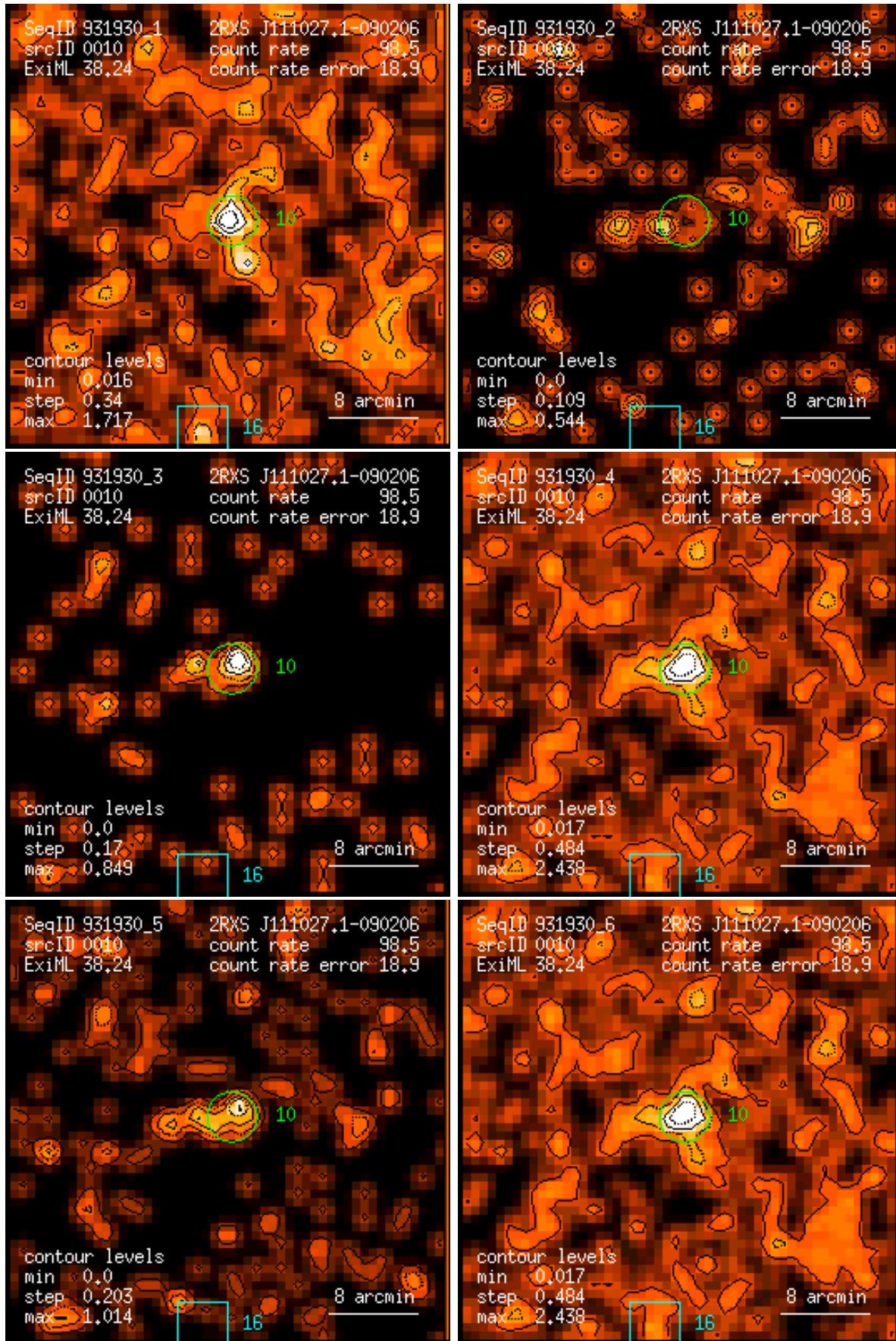
Figure 10: RASS 931930: detection 0010: band rate images, Gaussian filter: (1) PSPC channels 11 – 41, (2) 52 – 90, (3) 91 – 201, (4) 11 – 235, (5) 52 – 201, (6) 11 – 201. Broad band rates in counts/ks. Band rate contour levels in counts/ks/arcmin 2 .
