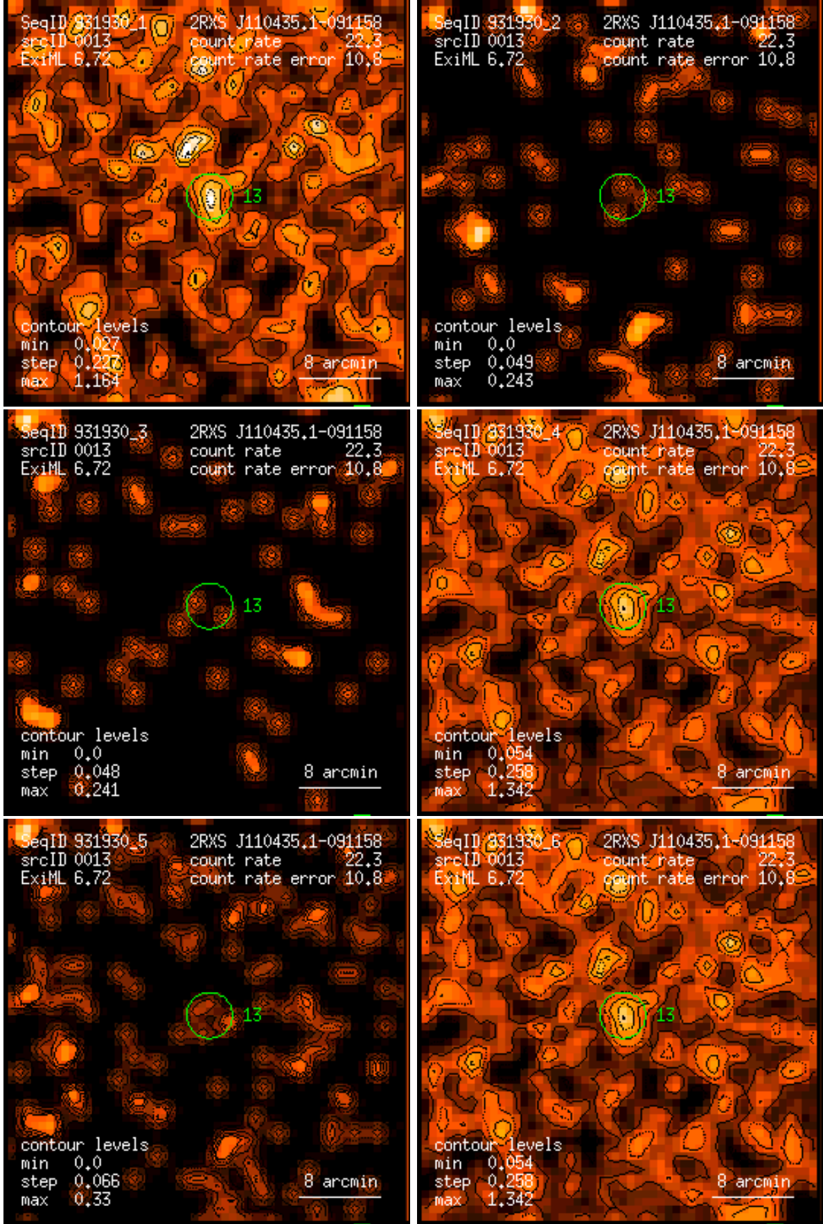
Figure 13: RASS 931930: detection 0013: band rate images, Gaussian filter: (1) PSPC channels 11 – 41, (2) 52 – 90, (3) 91 – 201, (4) 11 – 235, (5) 52 – 201, (6) 11 – 201. Broad band rates in counts/ks. Band rate contour levels in counts/ks/arcmin 2 .
