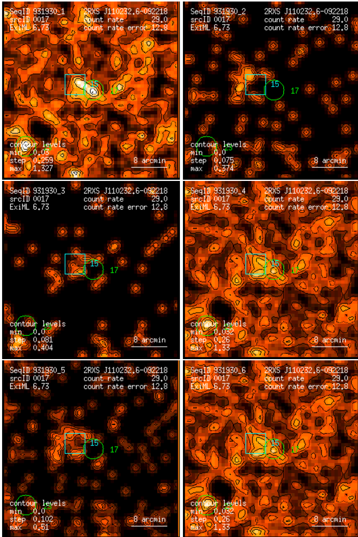
Figure 17: RASS 931930: detection 0017: band rate images, Gaussian filter: (1) PSPC channels 11 – 41, (2) 52 – 90, (3) 91 – 201, (4) 11 – 235, (5) 52 – 201, (6) 11 – 201. Broad band rates in counts/ks. Band rate contour levels in counts/ks/arcmin 2 .
