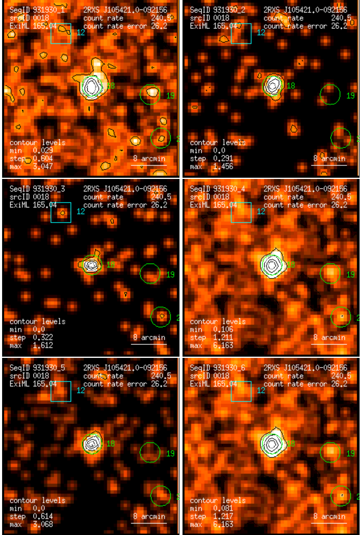
Figure 18: RASS 931930: detection 0018: band rate images, Gaussian filter: (1) PSPC channels 11 – 41, (2) 52 – 90, (3) 91 – 201, (4) 11 – 235, (5) 52 – 201, (6) 11 – 201. Broad band rates in counts/ks. Band rate contour levels in counts/ks/arcmin 2 .
