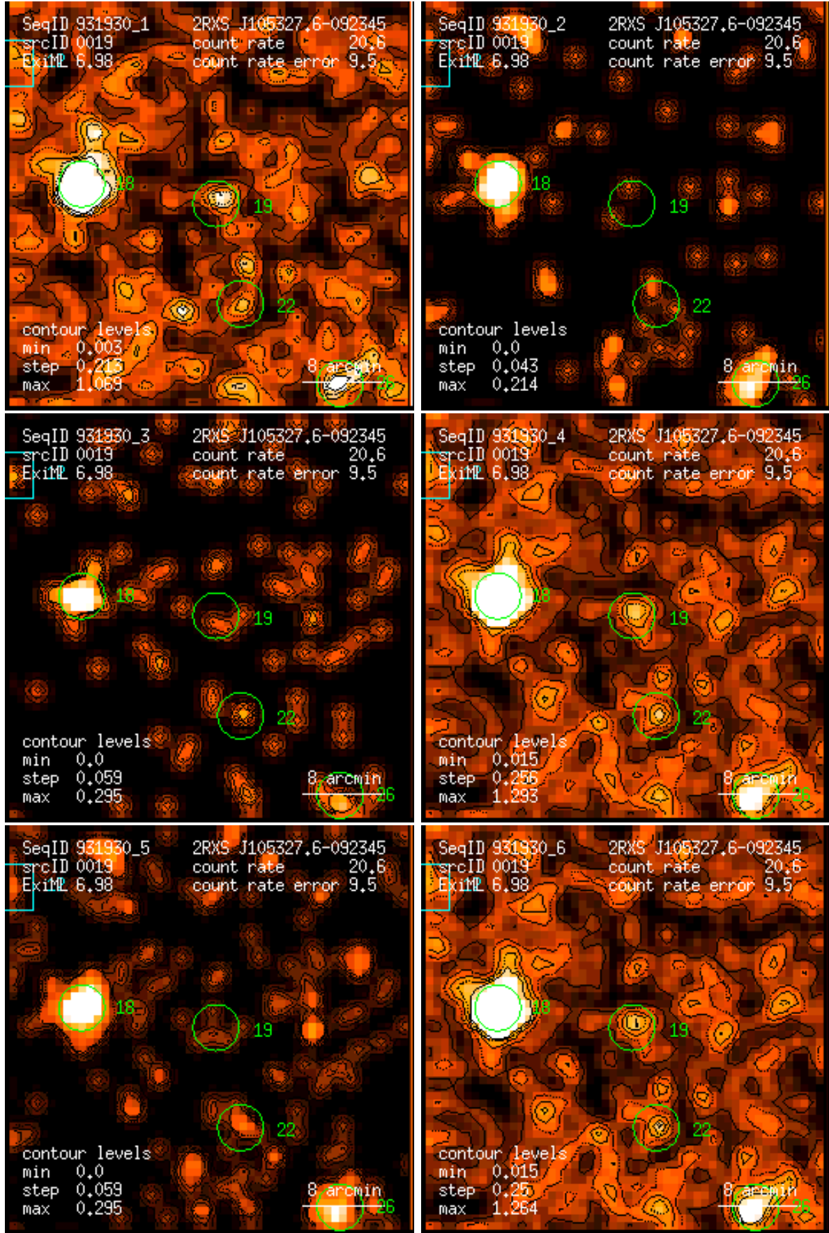
Figure 19: RASS 931930: detection 0019: band rate images, Gaussian filter: (1) PSPC channels 11 – 41, (2) 52 – 90, (3) 91 – 201, (4) 11 – 235, (5) 52 – 201, (6) 11 – 201. Broad band rates in counts/ks. Band rate contour levels in counts/ks/arcmin 2 .
