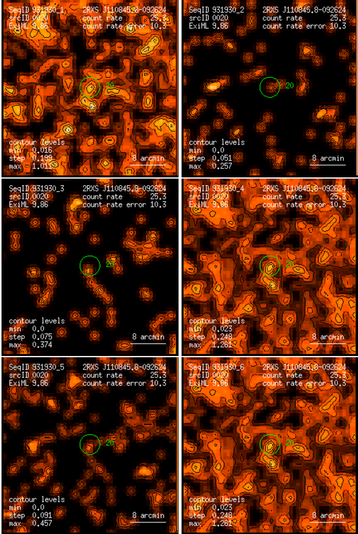
Figure 20: RASS 931930: detection 0020: band rate images, Gaussian filter: (1) PSPC channels 11 – 41, (2) 52 – 90, (3) 91 – 201, (4) 11 – 235, (5) 52 – 201, (6) 11 – 201. Broad band rates in counts/ks. Band rate contour levels in counts/ks/arcmin 2 .
