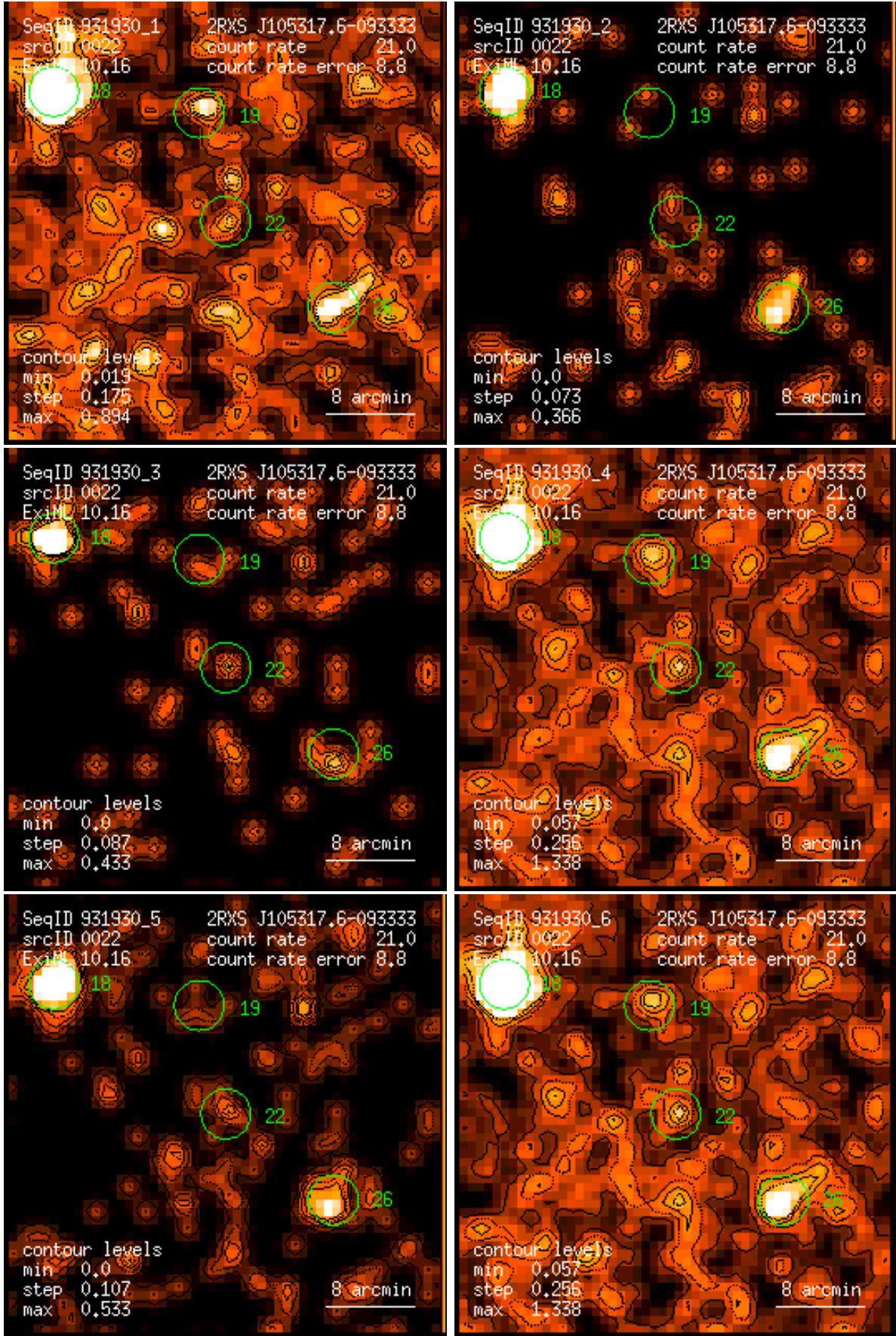
Figure 22: RASS 931930: detection 0022: band rate images, Gaussian filter: (1) PSPC channels 11 – 41, (2) 52 – 90, (3) 91 – 201, (4) 11 – 235, (5) 52 – 201, (6) 11 – 201. Broad band rates in counts/ks. Band rate contour levels in counts/ks/arcmin 2 .
