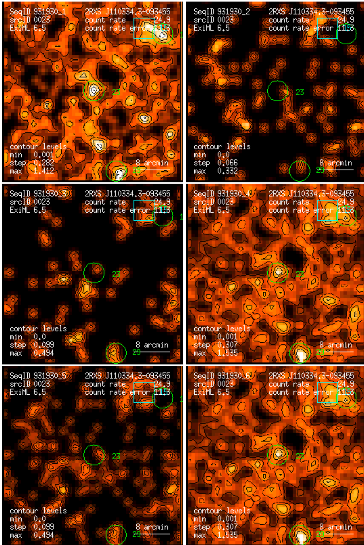
Figure 23: RASS 931930: detection 0023: band rate images, Gaussian filter: (1) PSPC channels 11 – 41, (2) 52 – 90, (3) 91 – 201, (4) 11 – 235, (5) 52 – 201, (6) 11 – 201. Broad band rates in counts/ks. Band rate contour levels in counts/ks/arcmin 2 .
